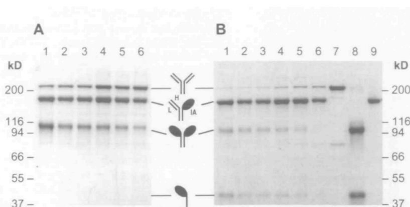
Fig. 2. SDS-PAGE analysis of protein A purified products from co-transfection of Ab H and L chains with IA for (A) wild-type chains and (B) Ab Y407T, IA T366Y variants. The ratio (by mass) of IA:H chain:L chain input DNAs (15 \mu g total) was varied as follows: lane 1, 8:1:3; lane 2, 7:1:3; lane 3, 6:1:3; lane 4, 5:1:3; lane 5, 4:1:3; lane 6, 3:1:3; lane 7, 1:0:0; lane 8, 0:1:3; and lane 9, sample from lane 5 after ion-exchange chromatography (mono S,
