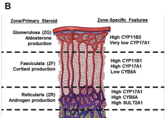
Fig. 1. (A) Major adrenal steroid synthesis pathways. (B) Adrenal zonation and enzyme expression pattern. SUL2A1/STS, steroid sulfotransferase type 2A1.
