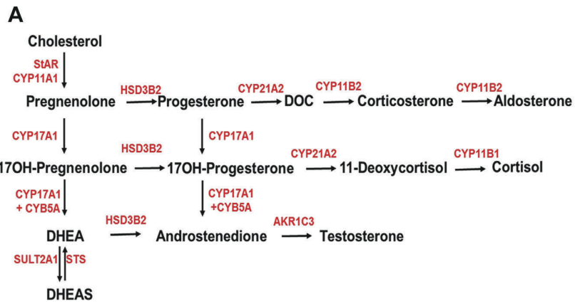
Fig. 1. (A) Major adrenal steroid synthesis pathways. (B) Adrenal zonation and enzyme expression pattern. SUL2A1/STS, steroid sulfotransferase type 2A1.
