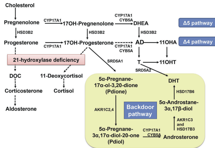
Fig. 2. Pathways of steroid hormone synthesis in 21-OHD, including backdoor pathway and 11-oxygenated androgens. AD, androstenedione; AKR1C2,4, aldo-keto reductase types 1C2 and 1C4; CYB5A, cytochrome b 5 ; CYP17A1, 17 \alpha -hydroxylase/17,20-lyase; DHEA, dehydroepiandrosterone; HSD17B6, 17 \beta -hydroxysteroid dehydrogenase type 6 (an oxidative 3 \alpha -HSD); SRD5A1/2, 5 \alpha -reductase, types 1 and 2; T, testosterone; 11OHA, 11 \beta -hydroxyandrostenedione; 11OHT, 11 \beta -hydroxytestosterone.
