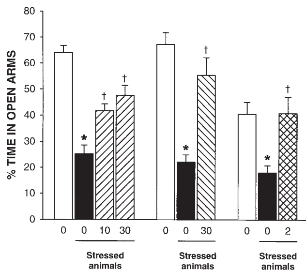
Fig. 5. Effects of SSR125543A (▨), antalarmin (⊞), and diazepam (⊞) on social defeat-induced anxiogenic-like behavior in the elevated plus-maze test in mice. Data represent mean \pm S.E.M. *, P < 0.05 versus non-stressed animals (□); †, P < 0.05 versus vehicle-treated stressed mice (▨); Newman-Keuls test. n = 8 to 10.
