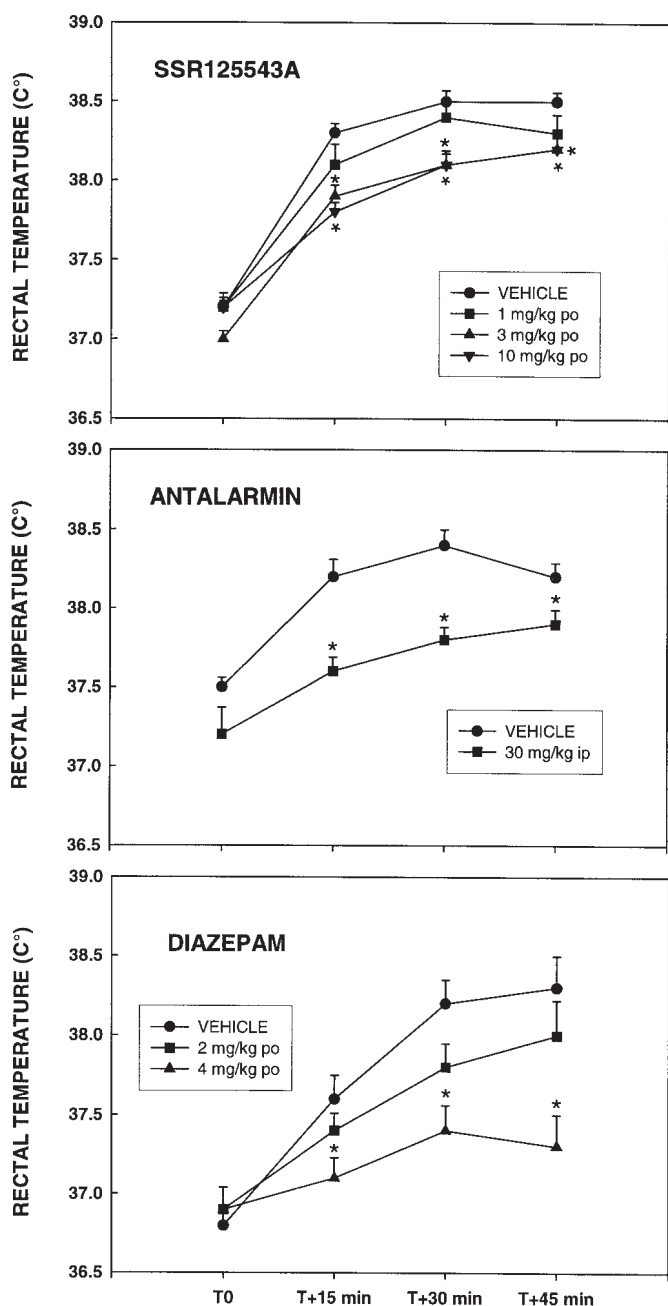
Fig. 2. Effects of SSR125543A, antalarmin, and diazepam on isolation stress-induced hyperthermia in rats. Data represent mean \pm S.E.M. \star , P < 0.05 (Dunnett's t test). n = 7 to 17.
