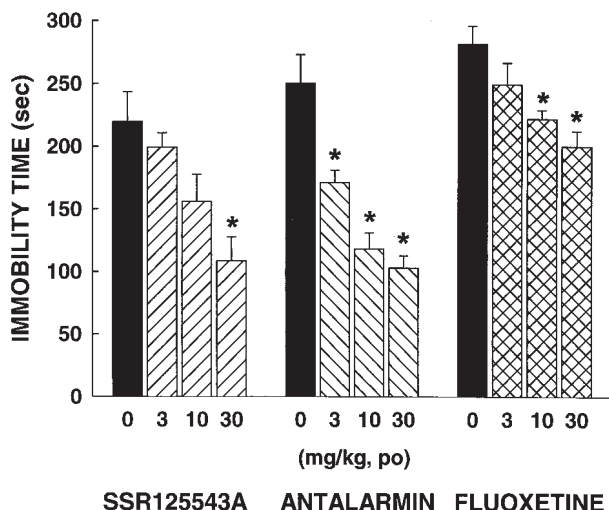
Fig. 6. Effects of SSR125543A, antalarmin, and fluoxetine in the forced swimming test in rats. Data represent mean \pm S.E.M. \star, P < 0.05 (Dunnett's t test). n = 6 to 7.
