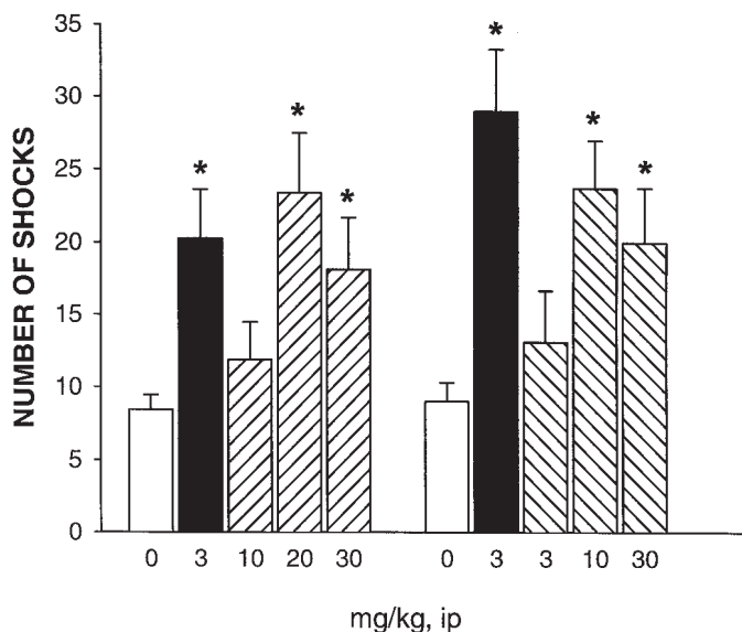
Fig. 1. Effects of diazepam (■), antalarmin (▨), and SSR125543A (▧) in the punished drinking conflict test in rats. Data represent mean \pm S.E.M. *, P < 0.05 (Dunnett's t test). n = 14 to 20.
