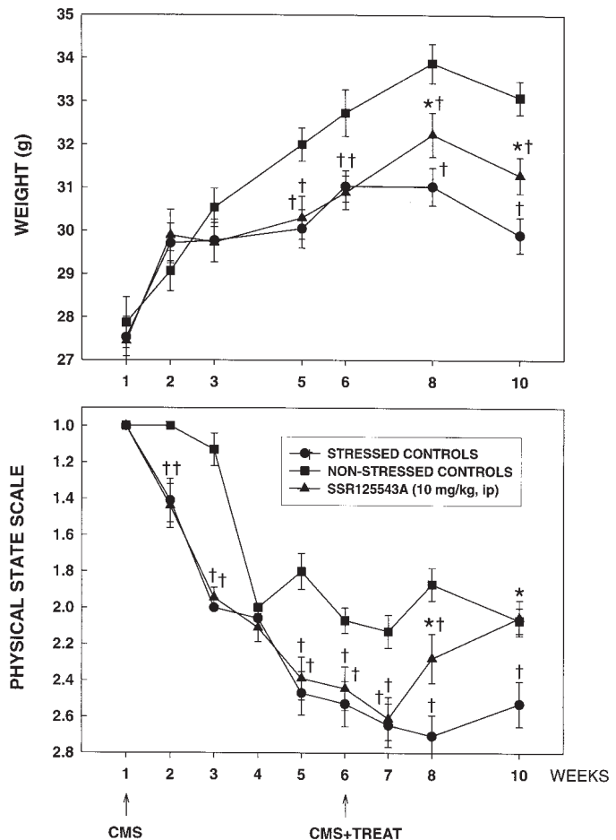
Fig. 7. Effects of repeated administration of SSR125543A on the reduction of body weight gain (top) and on the degradation of the physical state of the coat of animals (bottom) in chronically stressed (CMS) mice. Data represent mean \pm S.E.M. \star, P < 0.05 versus vehicle-treated stressed animals (●); \dagger, P < 0.05 versus nonstressed mice (■); Newman-Keuls test. n = 15 to 18.
