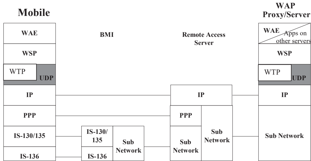
Figure 4-11: WDP over ANSI-136 Circuit-Switched Data
