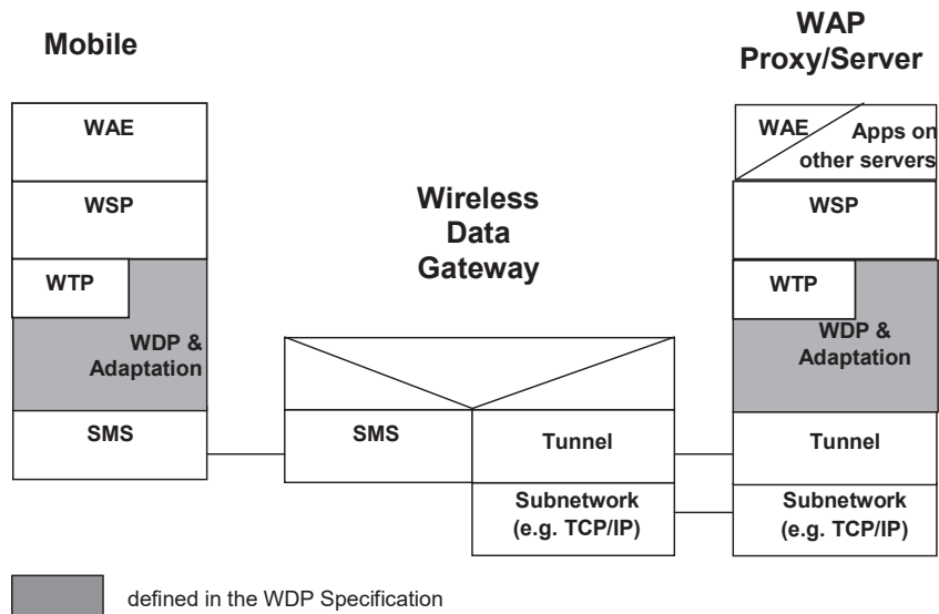
Figure 4-4 WDP over GSM SMS
