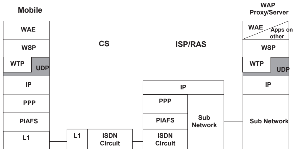
Figure 4-25 WDP over PHS Circuit-Switched Data Channel
