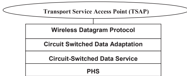
Figure 4-24 WDP over PHS Bearer Services
