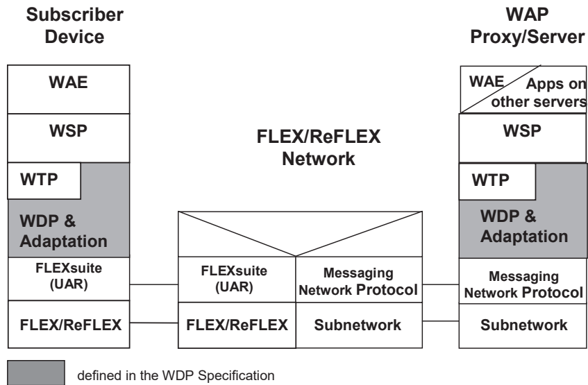
Figure 4-23 WDP over FLEX and ReFLEX
