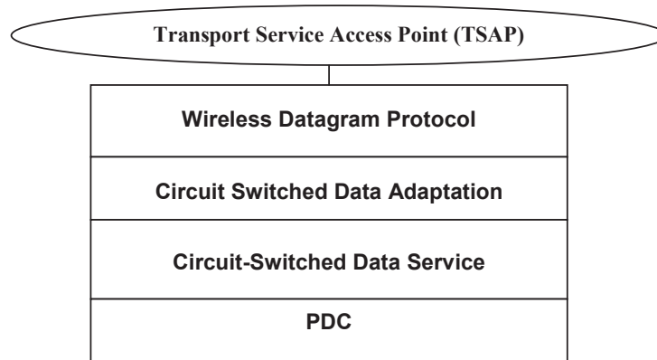
Figure 4-18: WDP over PDC Bearer Services
