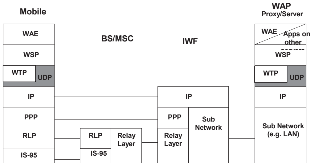
Figure 4-16 WDP over CDMA Packet Data Channel
