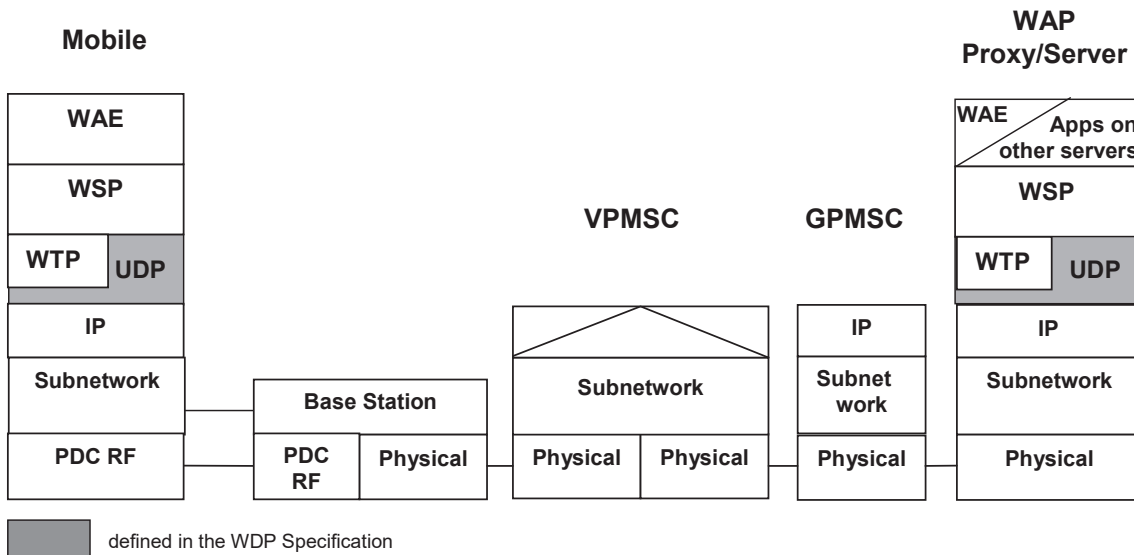
Figure 4-20 WDP over PDC Packet Data Channel
