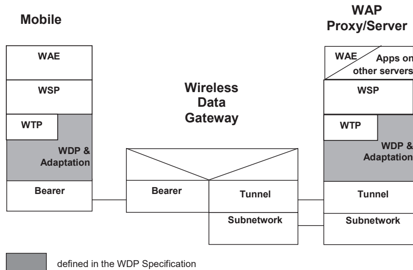
Figure 4-3 General WDP Architecture
