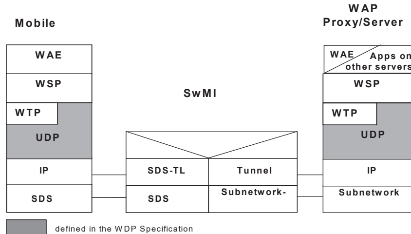
Figure 4-28 WDP over TETRA Packet Data
