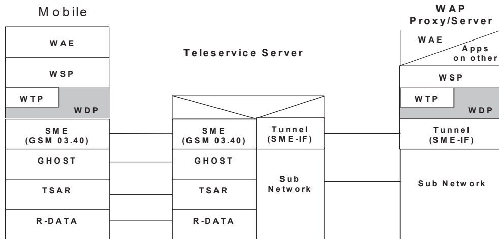
Figure 4-10 WDP over ANSI-136 R-DATA using GHOST
