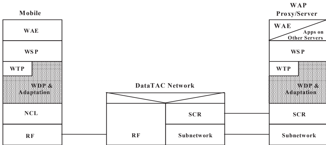
Figure 4-26: DataTAC Profile
