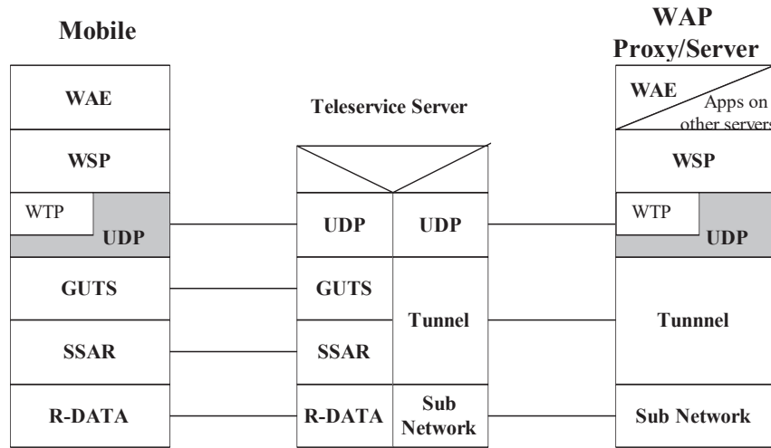
Figure 4-9: WDP over ANSI-136 R-DATA using GUTS
