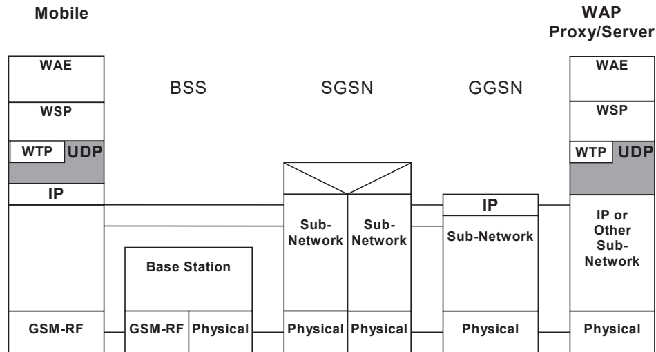
Figure 4-7 WDP over GSM GPRS
