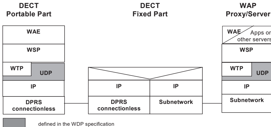
Figure 4-31: WDP over DECT packet switched services.
