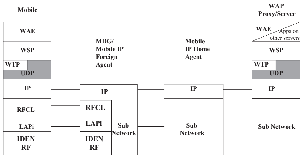
Figure 4-22: WTP over iDEN Packet Data
