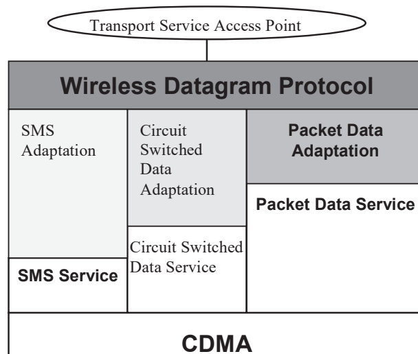
Figure 4-14: WDP over CDMA Bearer Services
