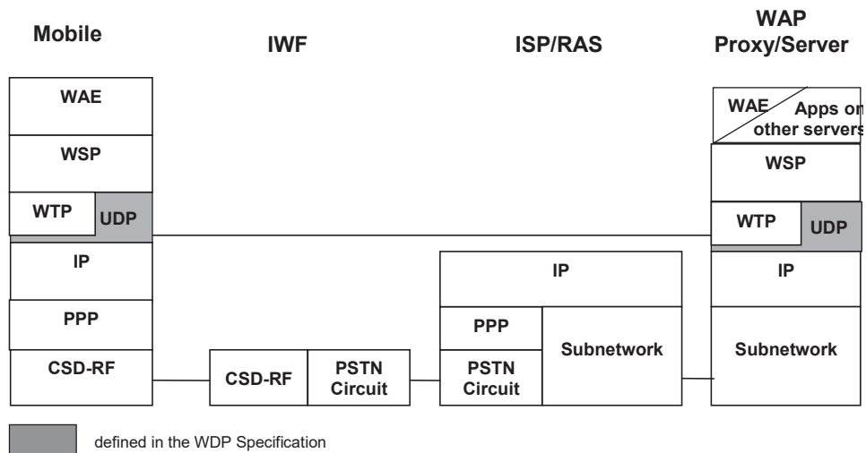
Figure 4-6 WDP over GSM Circuit Switched Data Channel
