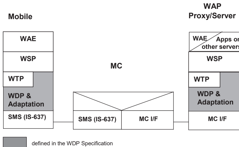
Figure 4-17 WDP over CDMA SMS
