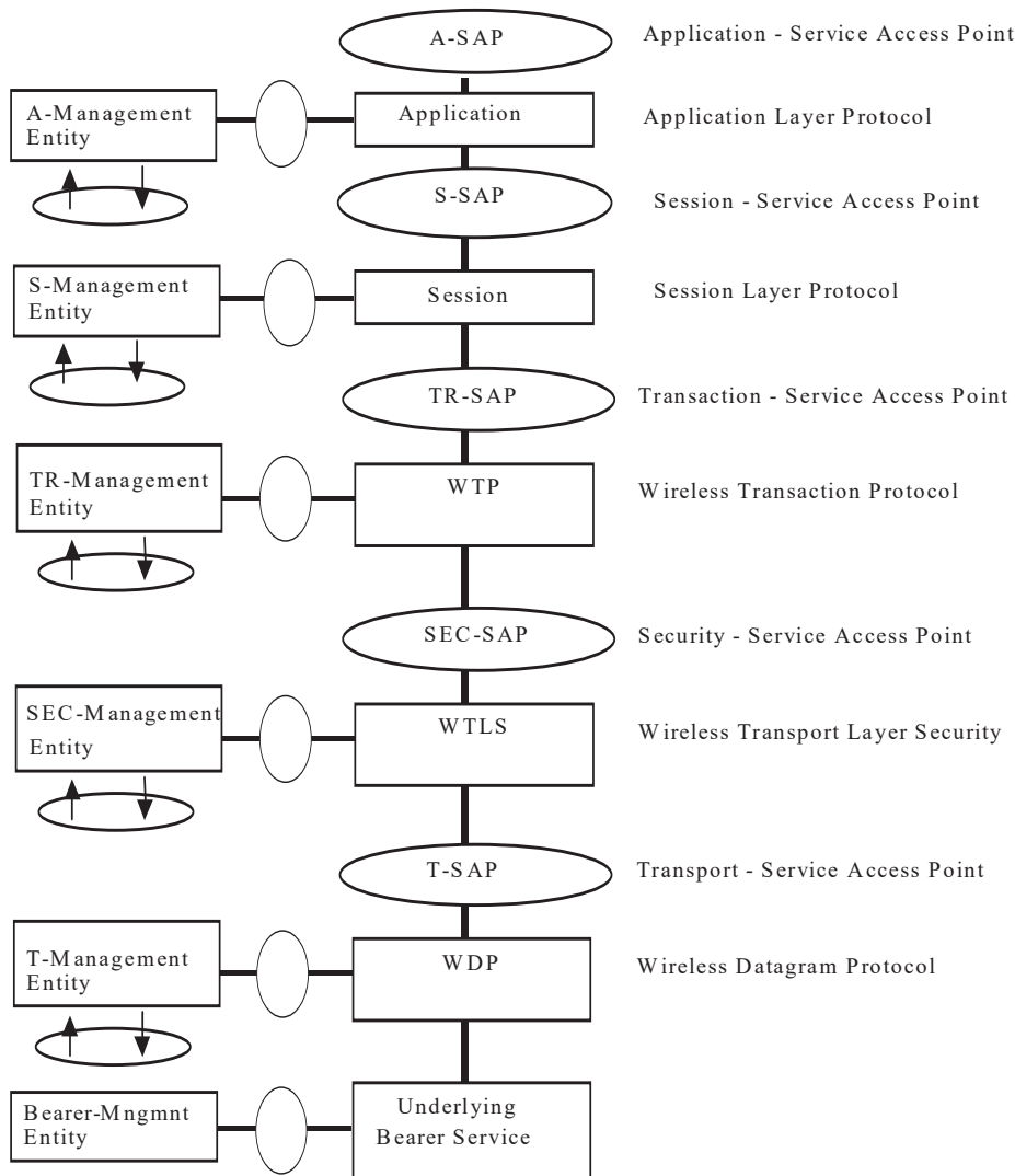
Figure 4-1 WAP Reference Architecture
