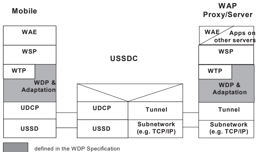
Figure 4-5 WDP over GSM USSD
