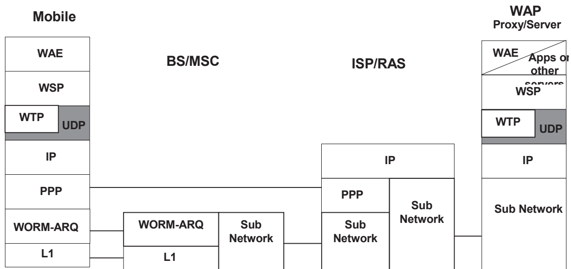
Figure 4-19 WDP over PDC Circuit-Switched Data Channel
