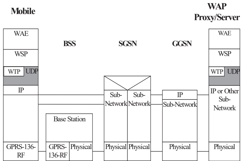
Figure 4-12: WDP over ANSI-136 Packet data
