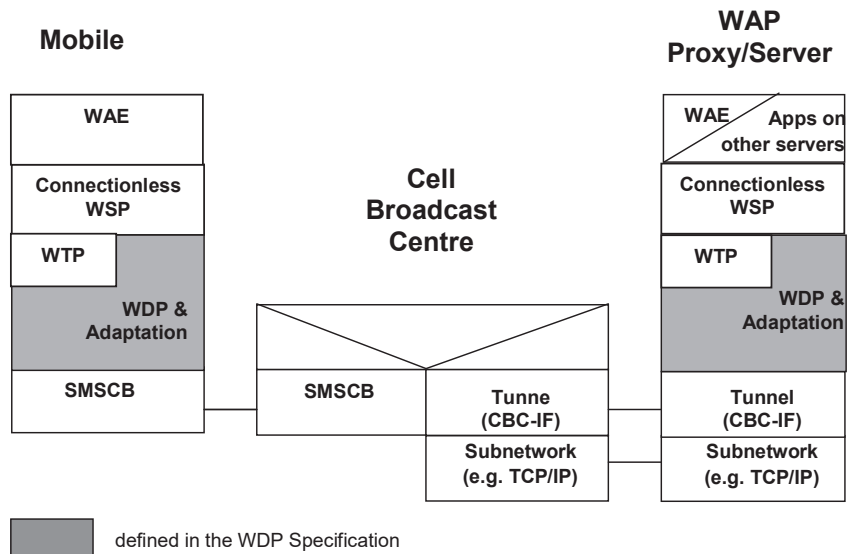
Figure 4-8 WDP over GSM Cell Broadcast
