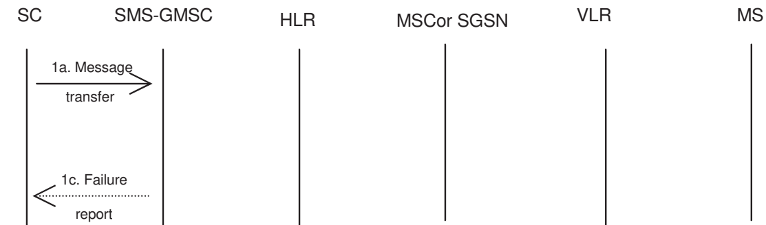
Figure 15a): Successful short message transfer attempt via the MSC or the SGSN
