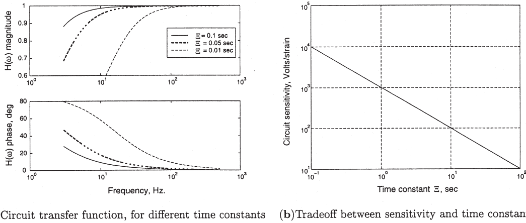
Figure 4. Circuit characteristics.
