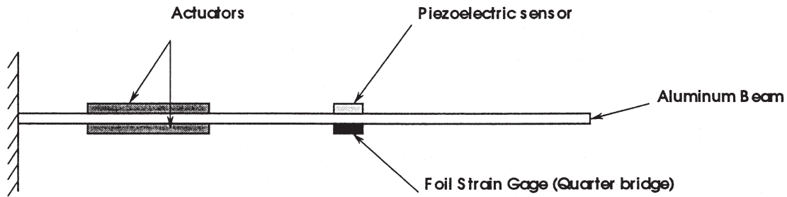
Figure 2. Calibration setup.
