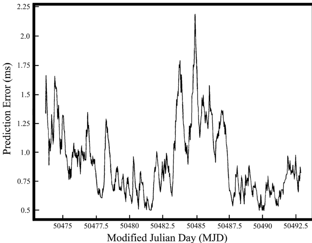
Figure 4. The uncertainty of the prediction (milliseconds) when the strain clock is synchronized to the server in Seattle. The long-period structure may be due to slow changes in the ambient temperature of the laboratory or to long-period fluctuations in the network delay.
