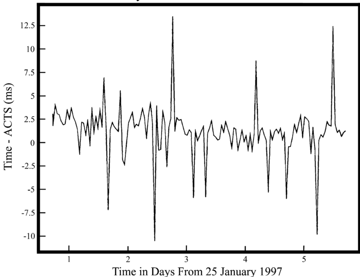
Figure 5. The time offset of the strain clock with respect to UTC as measured from the ACTS time signals. The ACTS comparisons are characterized by white phase noise of about 1 ms, so that fluctuations of that order or smaller are not significant.
