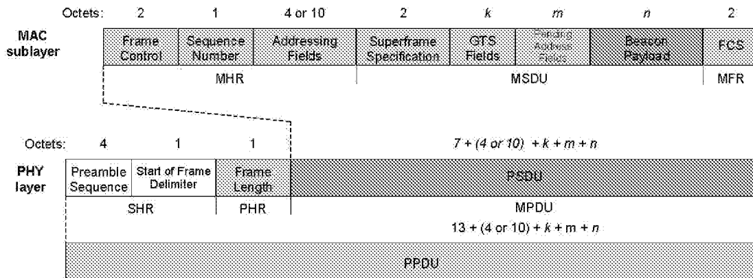
Figure 10—Schematic view of the beacon frame
