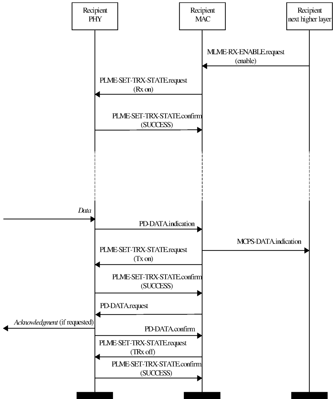
Figure 82—Data transmission message sequence chart—recipient
