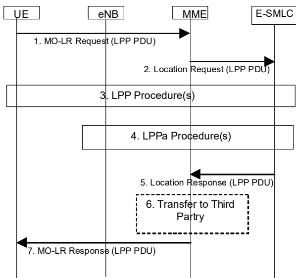
Figure 7.3.2-1: UE Positioning Operations to support an MO-LR
