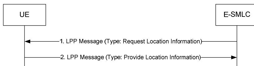
Figure 8.1.3-10: E-SMLC-initiated Position Measurement Procedure
