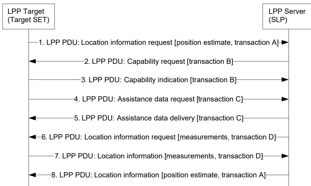
Figure B.4: LPP session over SUPL
