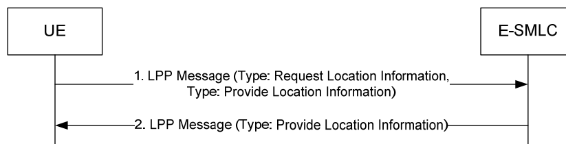
Figure 8.2.3-8: UE-initiated Position Measurement Procedure (Basic Self Location)
