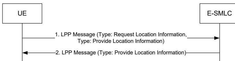
Figure 8.1.3-12: UE-initiated Position Measurement Procedure (Basic Self Location)
