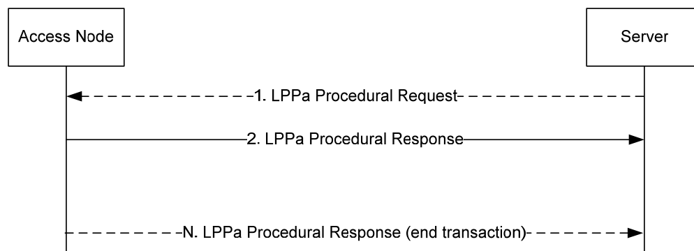
Figure 7.2.1-1: A single LPPa procedure
