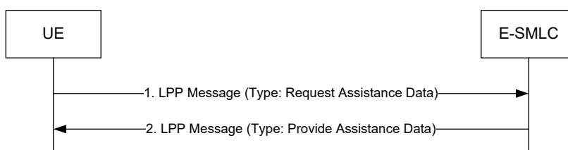
Figure 8.2.3-4: UE-initiated Assistance Data Delivery Procedure
