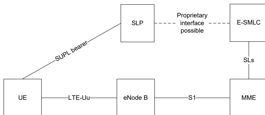
Figure 5-1: UE Positioning Architecture applicable to E-UTRAN
