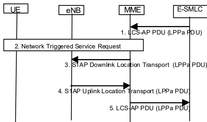
Figure 6.5.2-1: LPPa PDU Transfer between an E-SMLC and eNode B for UE Positioning
