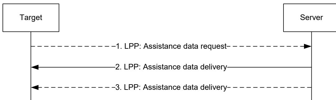
Figure 7.1.2-2: Assistance data transfer
