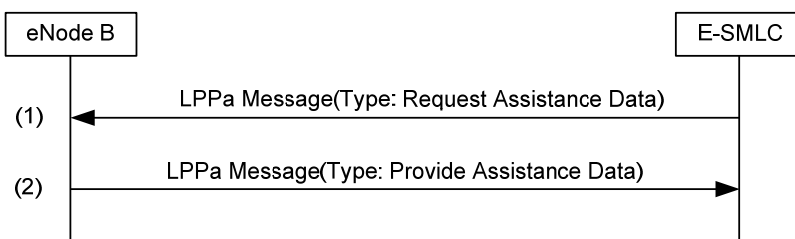
Figure 8.2.3-6: E-SMLC-initiated Assistance Data Delivery Procedure
