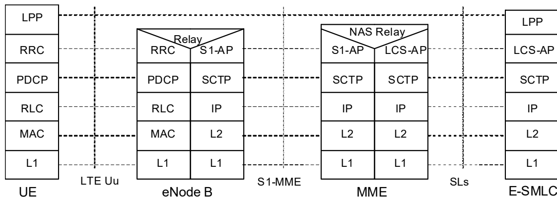
Figure 6.4.1-1: Protocol Layering for E-SMLC to UE Signalling
