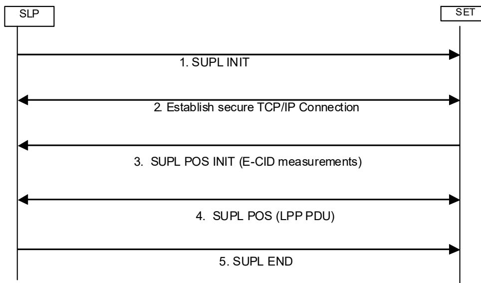
Figure B.3: LPP session over SUPL
