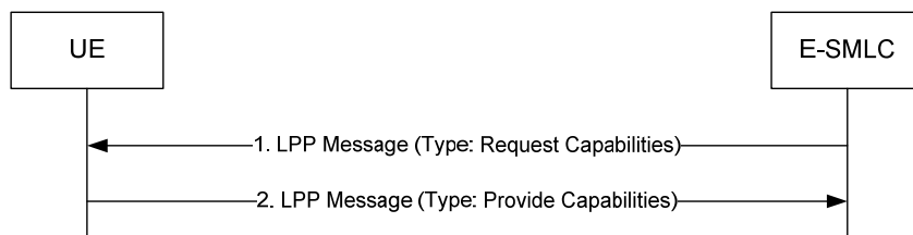
Figure 8.2.3-1: E-SMLC-initiated Position Capability Transfer
