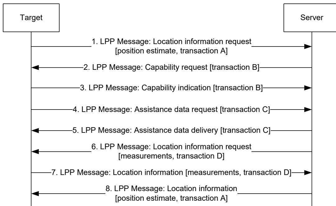
Figure 7.1.2-4: Example of multiple LPP procedures
