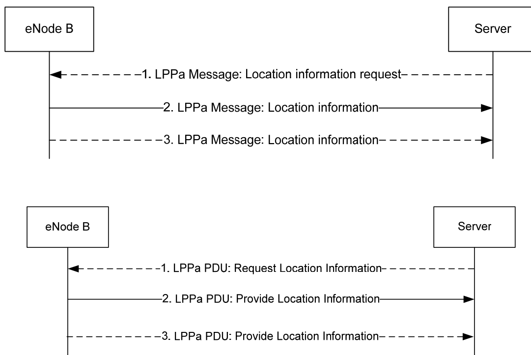
Figure 7.2.2-1: Location information transfer
