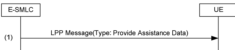
Figure 8.1.3-6: E-SMLC-initiated Assistance Data Delivery Procedure
