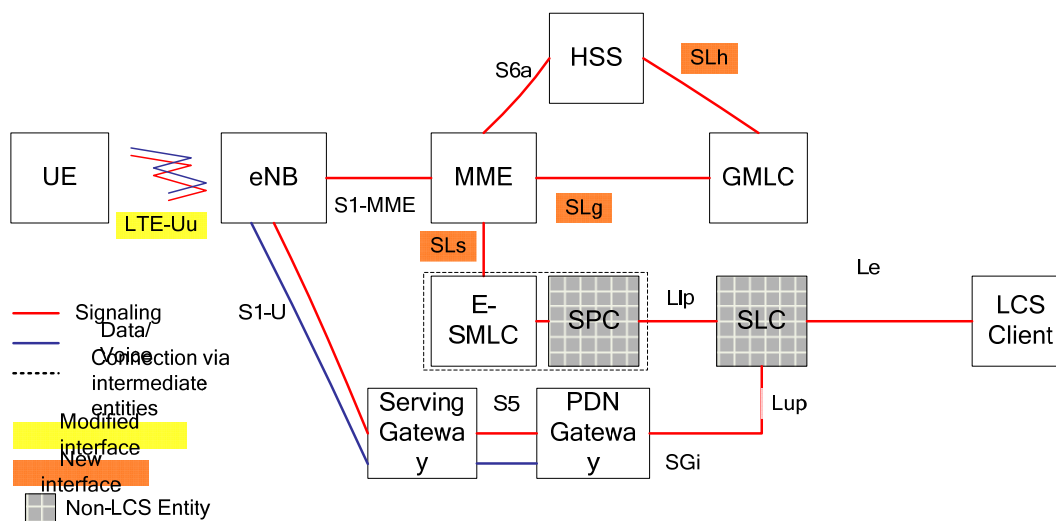
Figure B.1: System architecture underlying positioning
