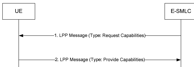
Figure 8.1.3-2: E-SMLC-initiated Position Capability Transfer
