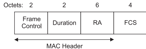
Figure 18—ACK frame
