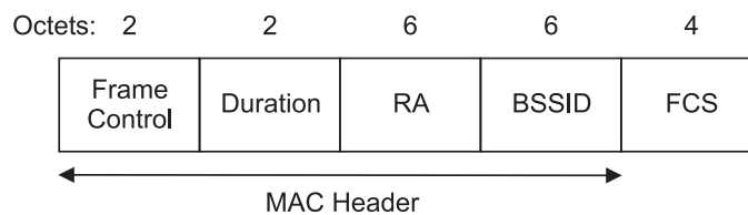
Figure 20—CF-End frame
