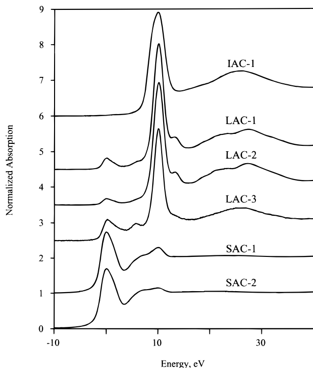
Figure 1. Sulfur K-edge XANES spectra of six activated carbon samples. Samples IAC-1, LAC-1, LAC-2, and SAC-1 were exposed to a synthetic flue gas (SFG) containing \text{SO}_2 , HCl, and \text{Hg}^0 .
