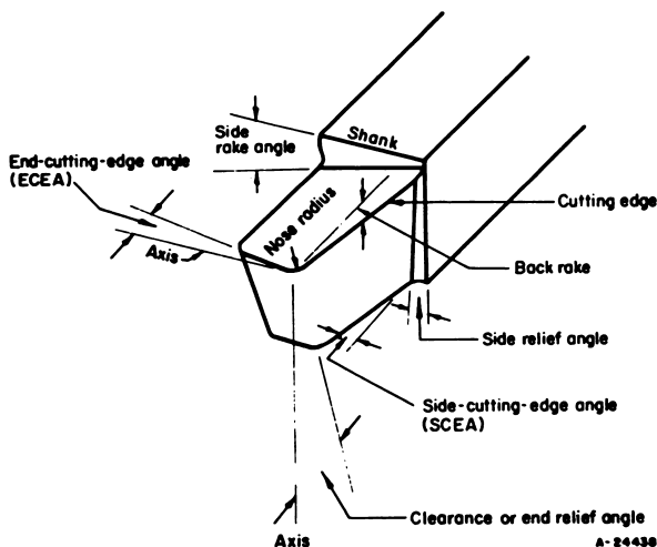
FIGURE 3. NOMENCLATURE FOR SINGLE-POINT CUTTING TOOLS
