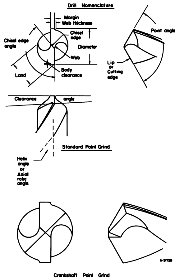
FIGURE 4. DRILL NOMENCLATURE AND ILLUSTRATION OF TWO TYPES OF DRILL-POINT GRINDS
