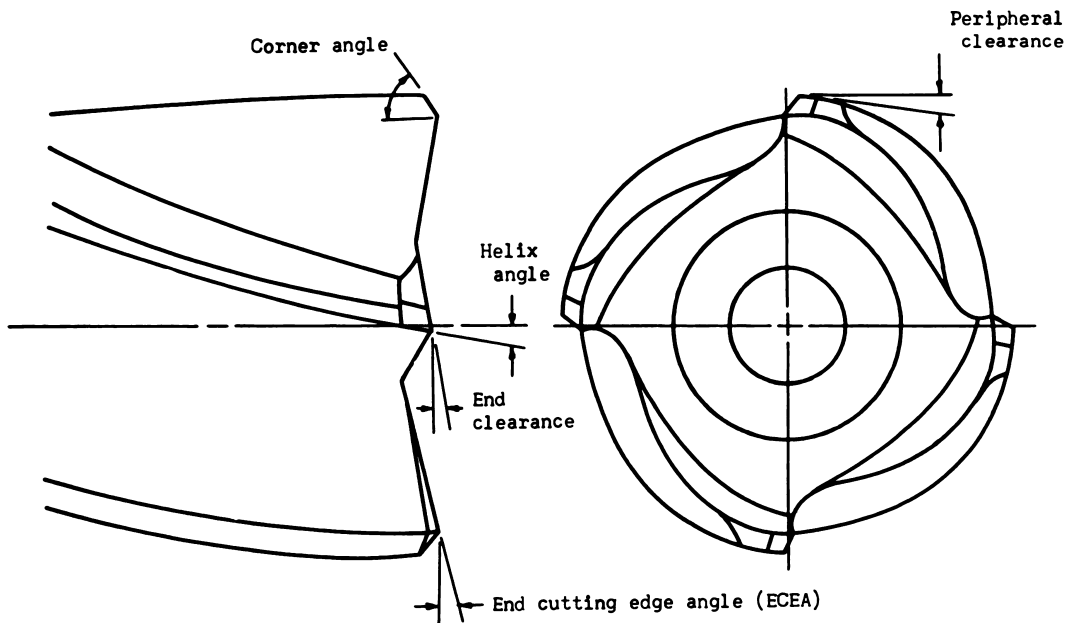
FIGURE 2. END-MILL NOMENCLATURE (7)
