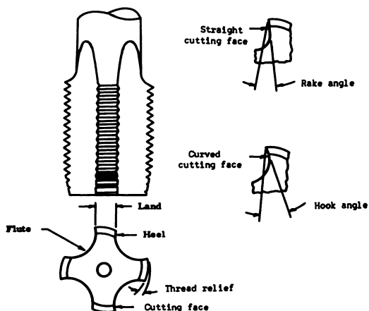
FIGURE 6. TAP NOMENCLATURE (8)
