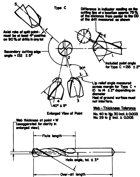
FIGURE 5. NAS 907 TYPE C AIRCRAFT DRILLS
