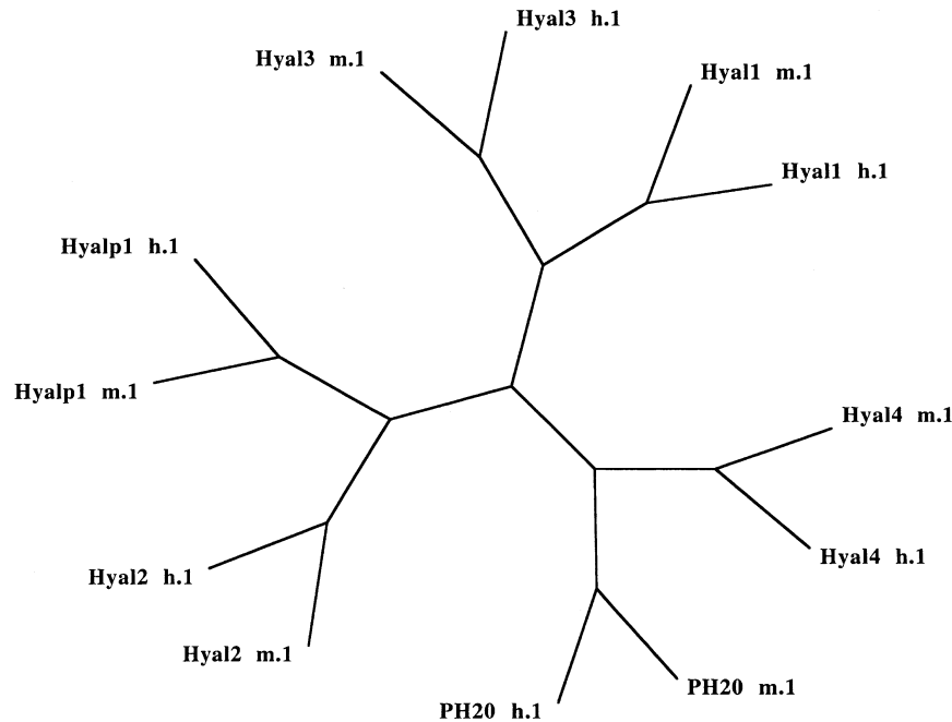
Fig. 5. Phylogenetic analysis of the 12 human and mouse hyaluronidases. h = human, m = mouse. The dendrogram was generated on the Bionavigator web site at http://www.bionavigator.com . Programs used to generate the dendrogram were ClustalW and Phylip (see text for references).
