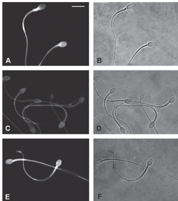
Fig. 3. Non-capacitated washed sperm were exposed to Limulus polyphemus (LPA), a lectin that specifically recognizes sialic acid (A, B). Two other lectins with known specificity to sialic acid, Maackia amurensis (MAL II, C, D) and Triticum vulgaris (WGA, E, F) also appeared to have the same uniform fluorescence pattern over the entire sperm surface as observed with LPA. The sialic acid lectins had the same uniform fluorescent pattern as the poly-L-lysine and histone labeling, which recognized the negatively charged surface molecules (see Fig. 2A–D). Bar = 10 \mu\text{m}
