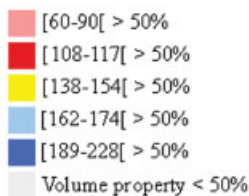
Plate 2. IMGT Collier de Perles statistical profile for volume. (A) Human IGHV and IGKV+IGLV. (B) Human IGKV and IGLV. The positions are shown with a volume profile defined at \geq 50\% and \geq 80\% threshold (see text). In (A), half circles correspond to IGHV (left) and IGKV + IGLV (right), and in (B), to IGKV (left) and IGLV (right).
