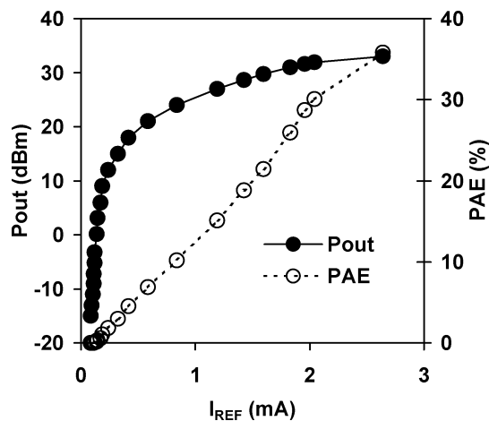
Fig. 14. GMSK PA characteristics showing output power ( P_{out} ) and PAE at 900 MHz and P_{in} = 14 dBm. High PAE is exhibited at high output power levels.
