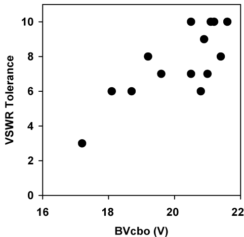
Fig. 1. PA VSWR tolerance at rated output power for process splits in a 0.5\text{-}\mu\text{m} SiGe HBT technology. Results show that the dc parameter BV_{cbo} is a useful metric for predicting device ruggedness in PA applications. PAs tested at V_c = 3.5\text{ V} , P_{out} = 35\text{ dBm} and f = 900\text{ MHz} .
