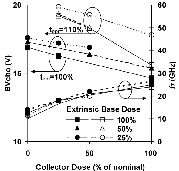
Fig. 2. Experimental results showing SiGe HBT device sensitivity in a 0.5\text{-}\mu\text{m} generation BiCMOS process. The experiment indicates that BV_{cbo} , an important measure of device ruggedness, can be modified significantly without perturbing f_T .
