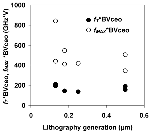
Fig. 9. Observed speed–ruggedness tradeoff for four lithographic generations of high-breakdown SiGe HBTs, from both production and experimental technologies. These results suggest that technology scaling will enhance PA device performance primarily through improvements in f_{MAX} , although improvements in the f_T \cdot BV_{ceo} metric are observed at the 0.13- \mu\text{m} generation.
