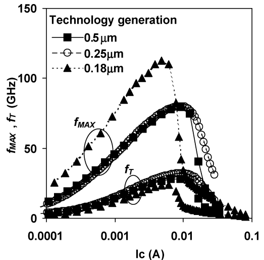
Fig. 8. AC characteristics of 2 \times 0.5 \mu\text{m} \times 20 \mu\text{m} high-breakdown SiGe HBTs at V_{cb} = 3 V from three lithographic generations. The 0.5-, 0.25-, and 0.18- \mu\text{m} technology devices have a BV_{ceo} of 7, 5.7, and 6 V, respectively.
