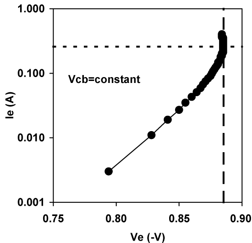
Fig. 6. Derivation of HBT instability points for determination of device SOA. The point at which the I_e - V_e curve attains a vertical slope for a fixed V_{cb} determines the maximum current at which the HBT can safely operate.
