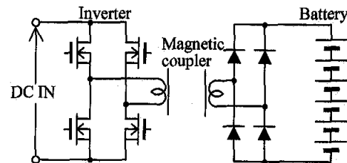
Fig. 1 Inductive charging for EV applications.
