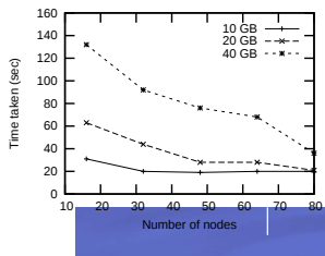
Figure 2: DEDUCE performance for I/O bound job
