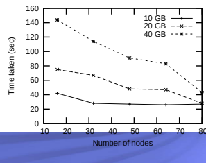
Figure 3: Hadoop performance for I/O bound job
