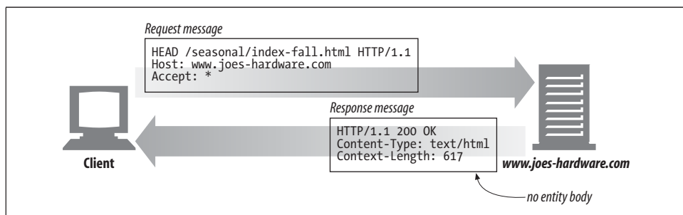
Figure 3-8. HEAD example
