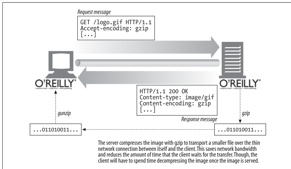
Figure 15-4. Content encoding
