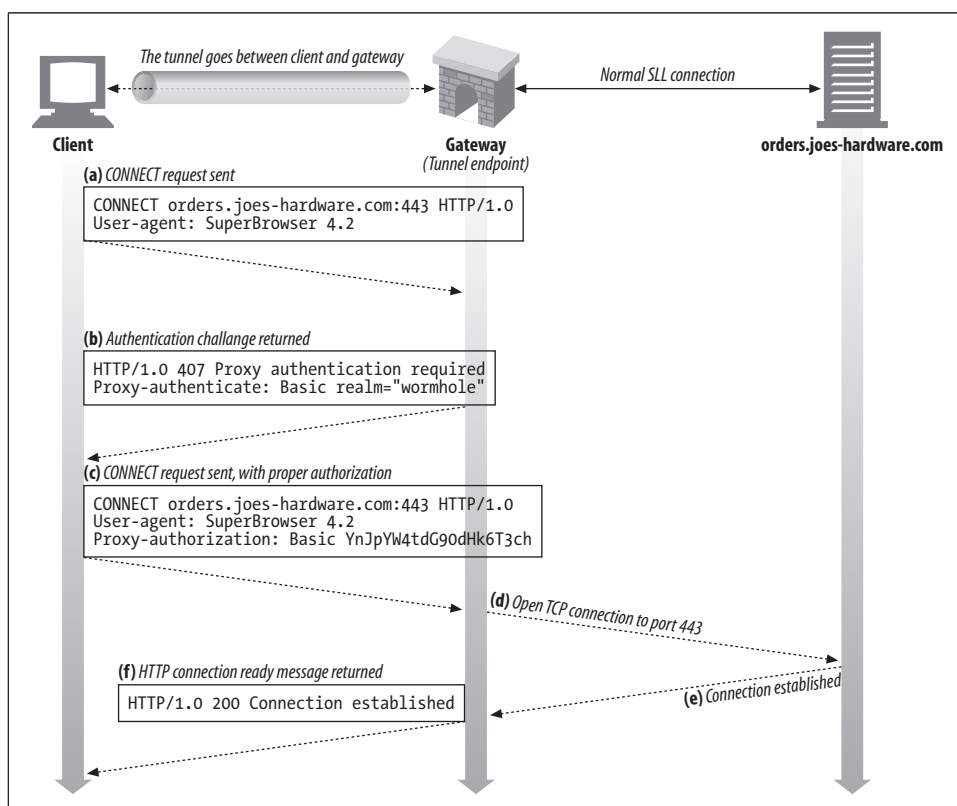
Figure 8-13. Gateways can proxy-authenticate a client before it's allowed to use a tunnel
