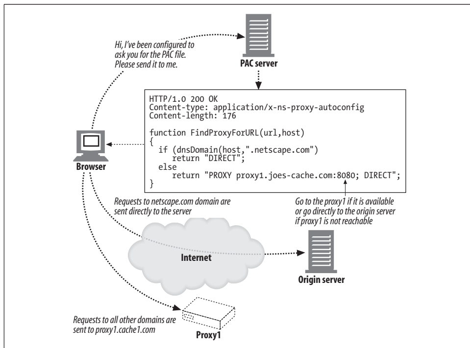
Figure 20-10. Proxy auto-configuration
