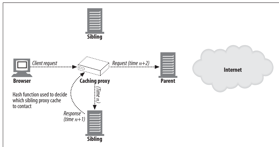
Figure 20-14. CARP redirection
