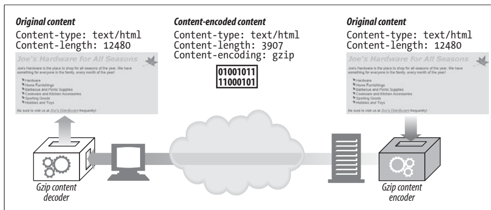
Figure 15-3. Content-encoding example
