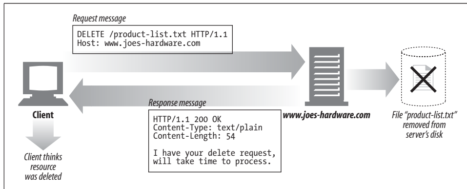
Figure 3-13. DELETE example
