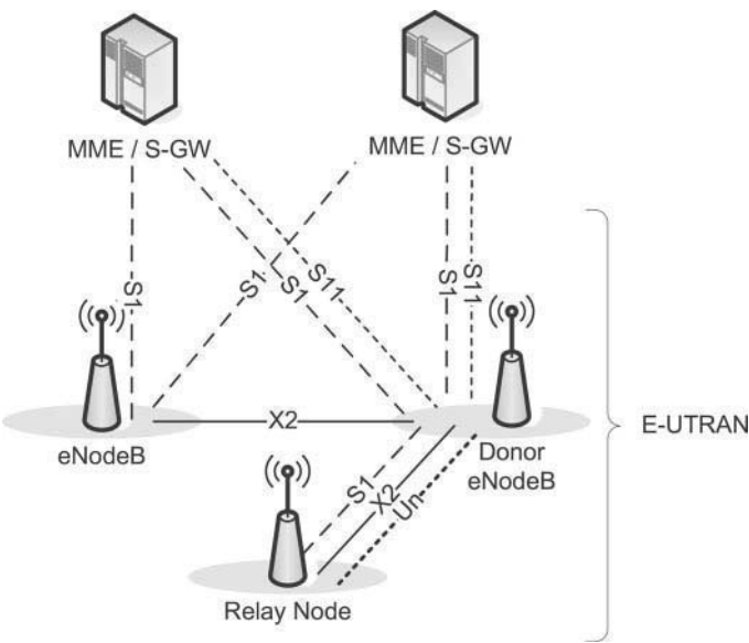
Figure 30.10: Network architecture and interfaces for RNs. Reproduced by permission of © 3GPP.
