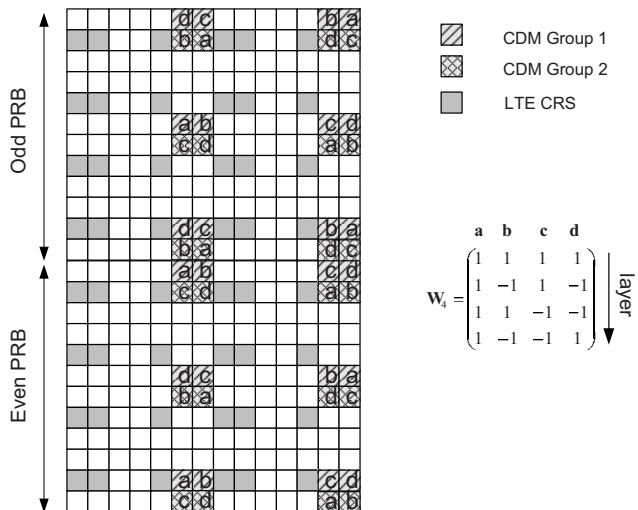
Figure 29.2: Length-4 OCC mapping to REs.
