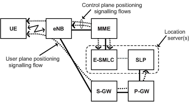
Figure 19.8: CP and UP architecture for positioning.
