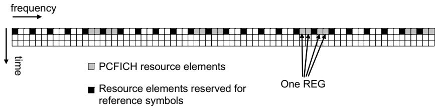
Figure 9.6: PCFICH mapping to Resource Element Groups (REGs).
