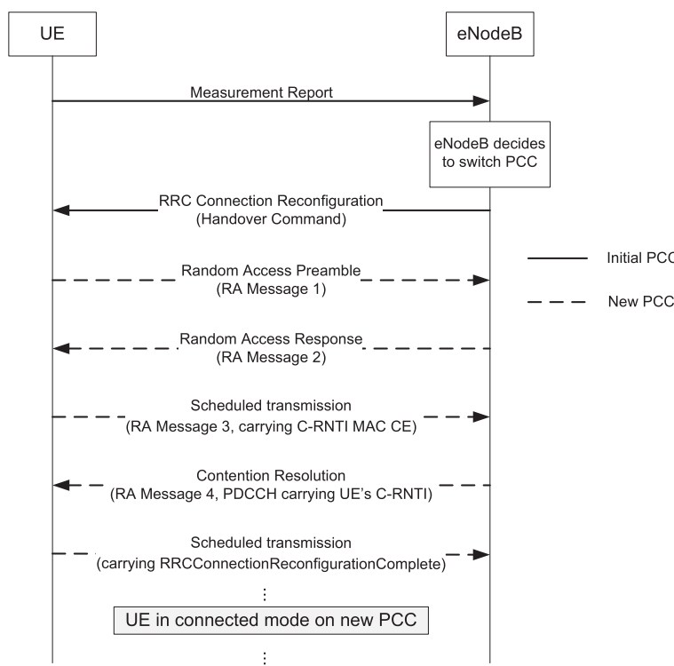
Figure 28.1: Procedure for PCell change with contention-based handover.
