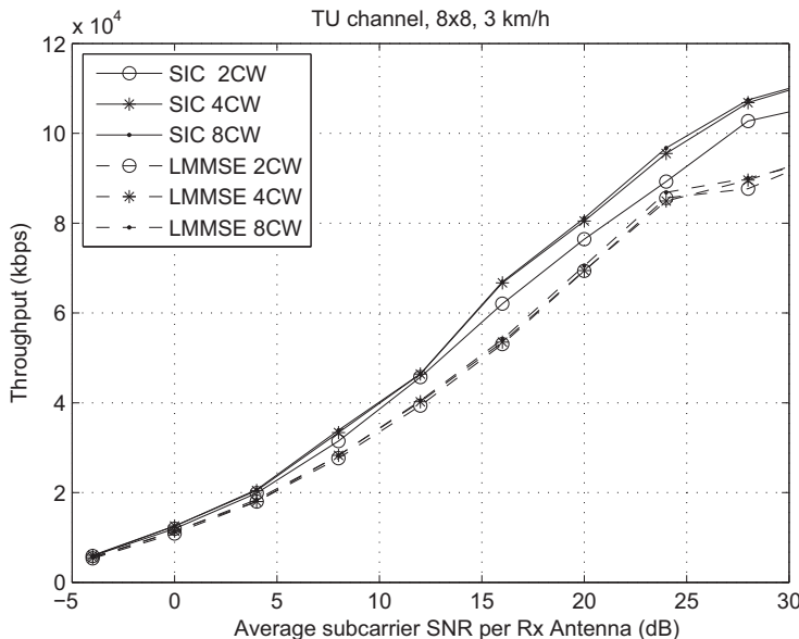
Figure 29.6: Throughput performance of LMMSE and MMSE-SIC receivers with different numbers of codewords.
