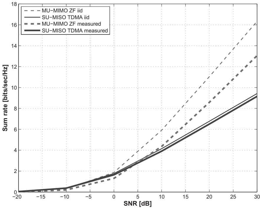
Figure 11.6: Ergodic sum-rate capacity of SU-MISO TDMA and MU-MIMO with two UEs, for an i.i.d. Rayleigh fading channel and for a measured channel.
