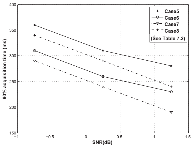
Figure 22.4: Cell search performance with unsynchronized eNodeBs. Reproduced by permission of © NXP Semiconductors.
