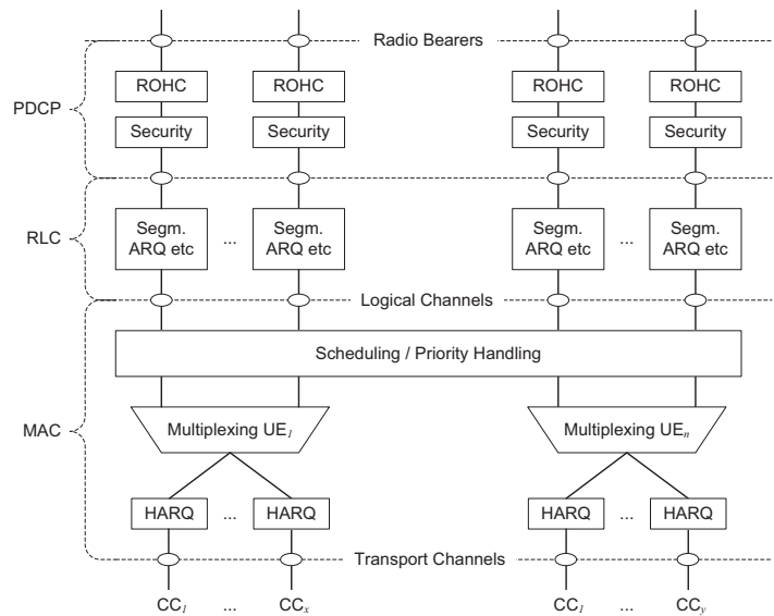
Figure 28.3: Downlink Layer 2 protocol structure for carrier aggregation. Reproduced by permission of © 3GPP.
