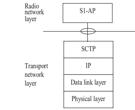
Figure 2.13: S1-MME control plane protocol stack. Reproduced by permission of © 3GPP.
