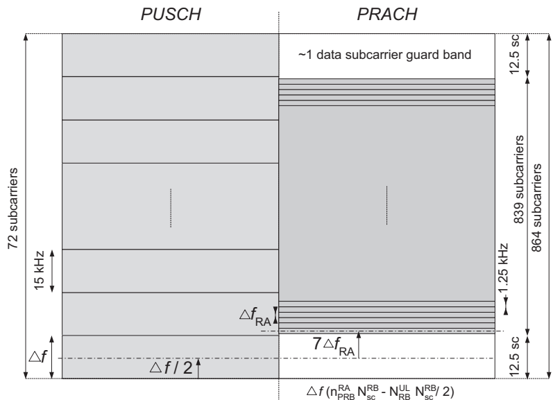
Figure 17.14: PRACH preamble mapping onto allocated subcarriers.
