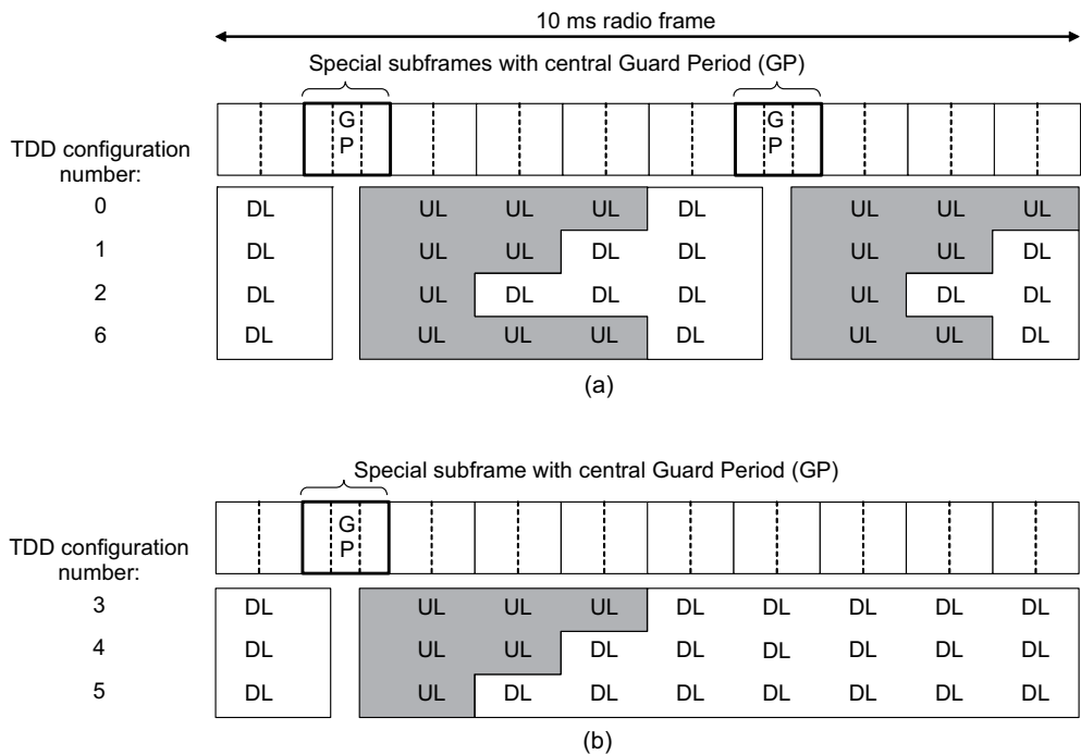
Figure 6.2: LTE subframe structure for TDD operation:
