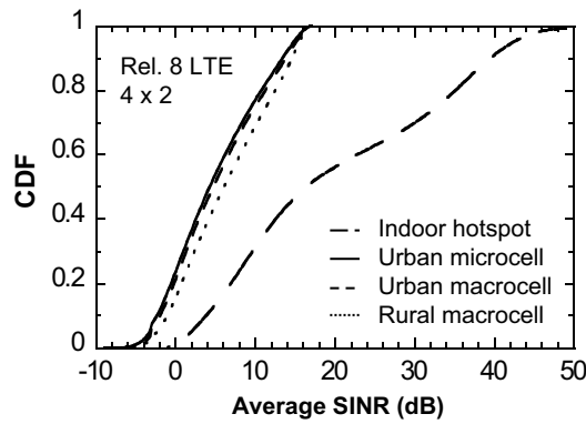
Figure 26.4: Downlink received SINR distribution for the ITU-R deployment scenarios.
