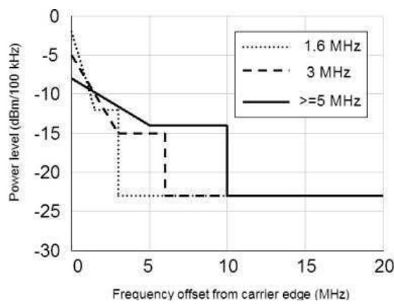
Figure 21.7: Spectrum emission mask for eNodeB transmitter.
