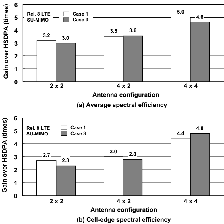
Figure 26.1: Ratio of Release 8 LTE FDD and HSDPA downlink spectral efficiencies for the Case 1 and Case 3 deployment scenarios.
