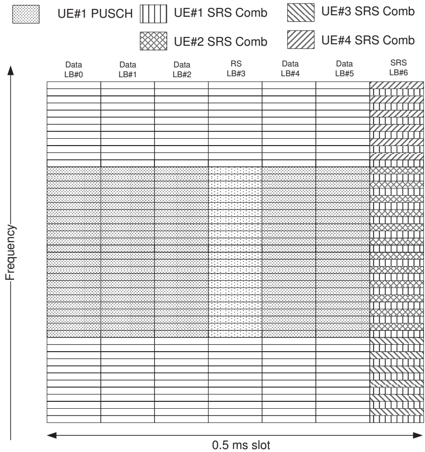
Figure 15.9: SRS symbol structure with RPF = 2.
