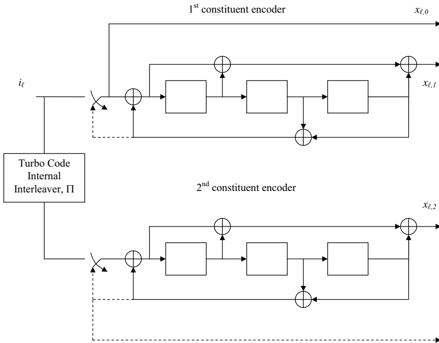
Figure 10.6: Schematic view of parallel turbo code used in LTE and UMS [10]. Reproduced by permission of © 3GPP.
