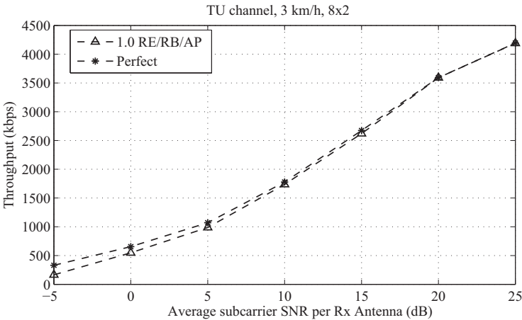
Figure 29.3: Throughput performance with a CSI-RS density of 1 RE per RB per antenna port: uncorrelated 8×2 SU-MIMO, 5 MHz, Typical Urban channel model, 3 km/h.
