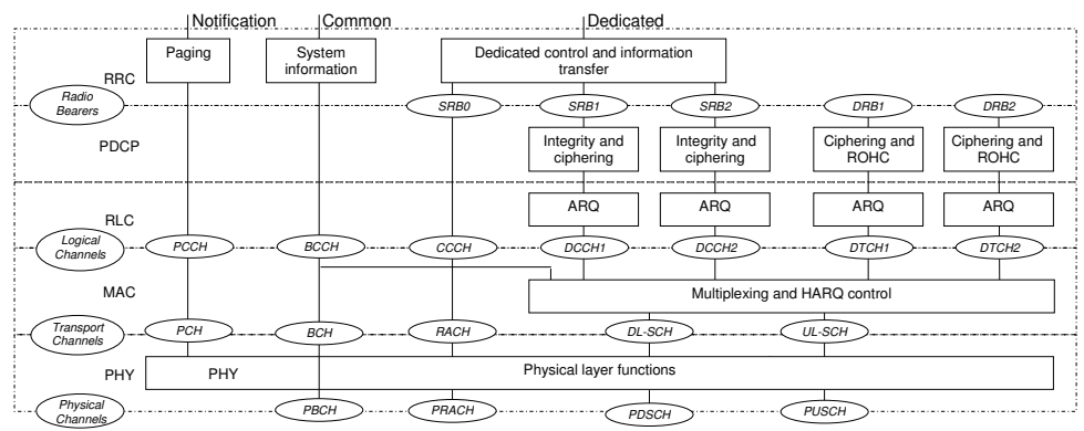
Figure 3.1: Radio architecture.
