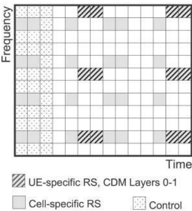
Figure 8.6: Dual-layer UE-specific RS arrangement in Release 9.
