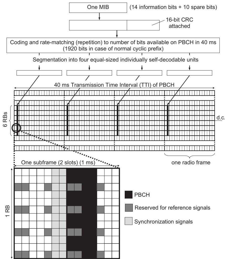
Figure 9.1: PBCH structure.
