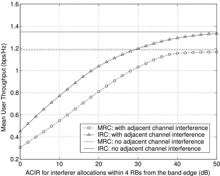
Figure 23.7: Comparison of IRC and MRC receivers with and without adjacent channel UE-UE interference.
