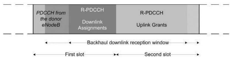
Figure 30.14: Placement of the R-PDCCH.
