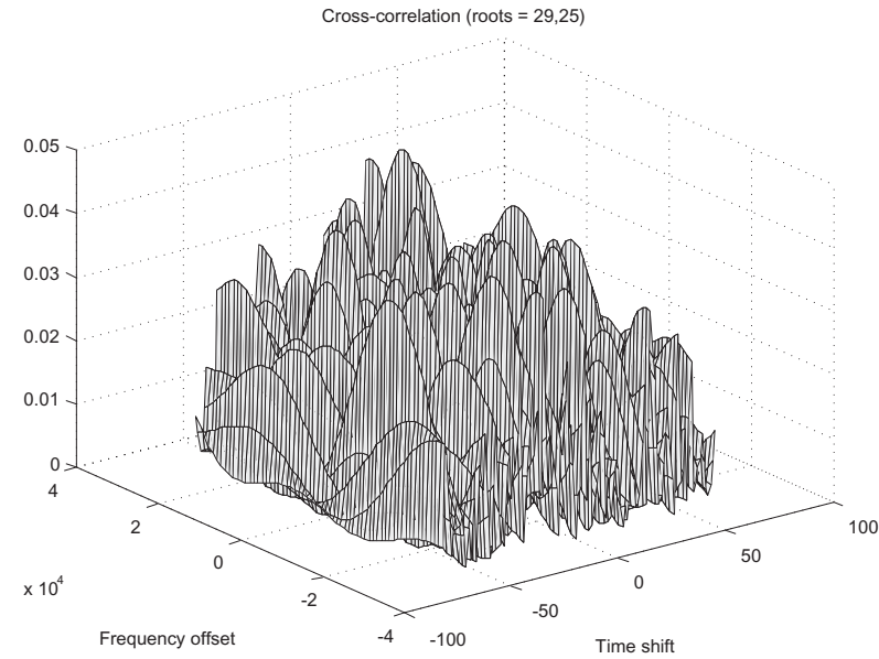
Figure 7.8: Cross-correlation of the PSS sequence pair 25 and 29.
