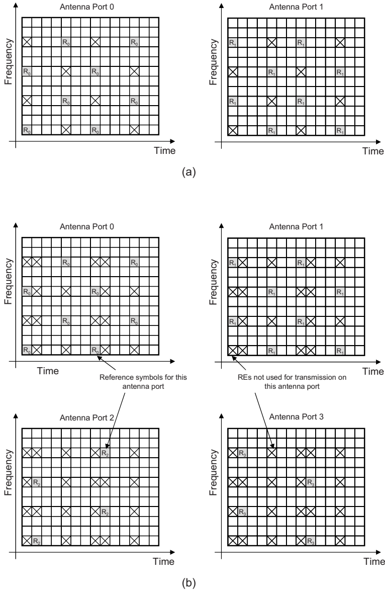
Figure 8.3: Cell-specific RS arrangement in the case of normal CP length for (a) two antenna ports, (b) four antenna ports. Reproduced by permission of © 3GPP.
