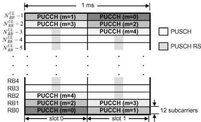
Figure 16.7: Example of an odd number of PUCCH regions ( N_{\text{RB}}^{\text{HO}} = 5 ).
