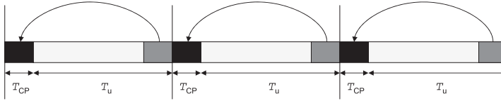
Figure 5.5: OFDM Cyclic Prefix (CP) insertion.
