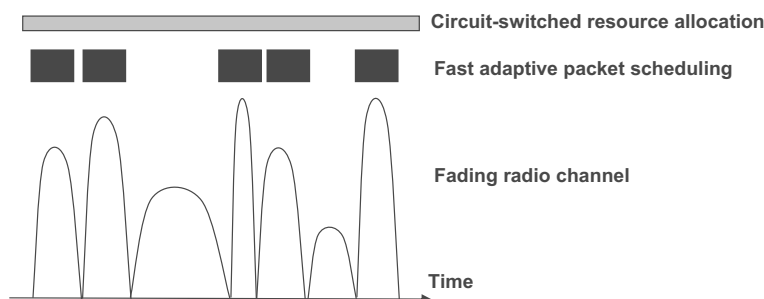
Figure 1.6: Fast scheduling and link adaptation.
