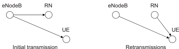
Figure 30.8: Cooperative operation of Type 2 RNs.
