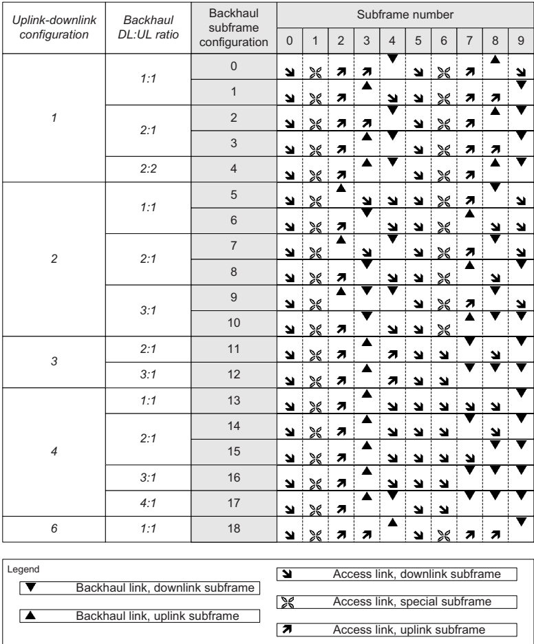
Figure 30.17: TDD subframe configurations.
