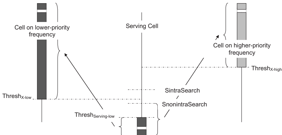
Figure 3.13: Frequency/RAT evaluation.
