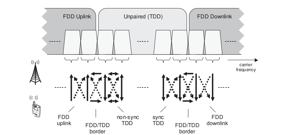
Figure 23.3: Possibilities for Adjacent Carrier Interference (ACI) between FDD and TDD systems.
