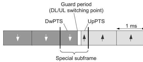
Figure 23.10: Special subframe for downlink–uplink switching in TDD operation.
