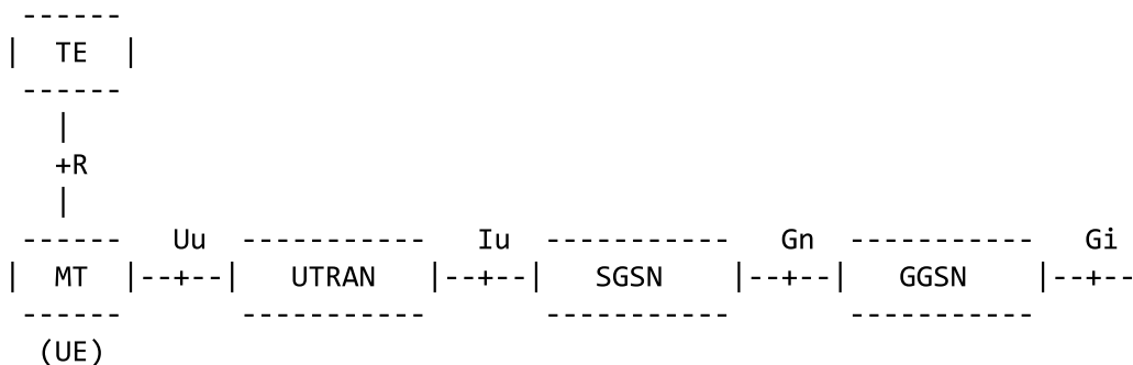
Figure 1: Simplified GPRS Architecture
