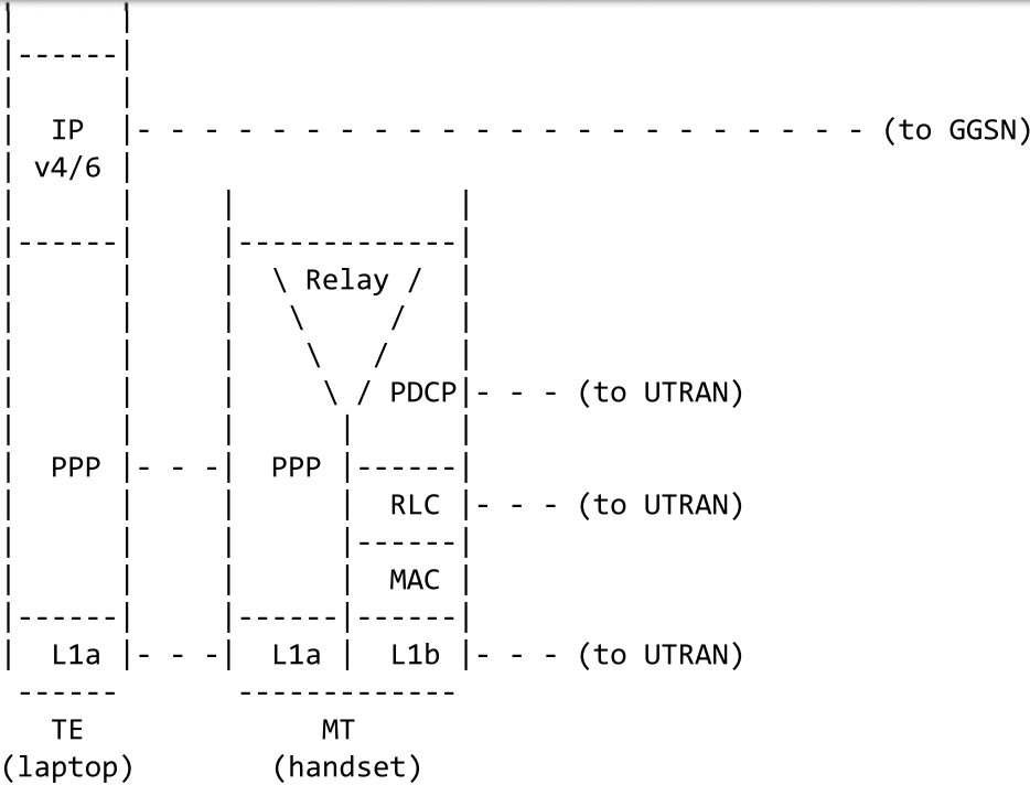
Figure 3: Laptop Attached to 3GPP Handset
