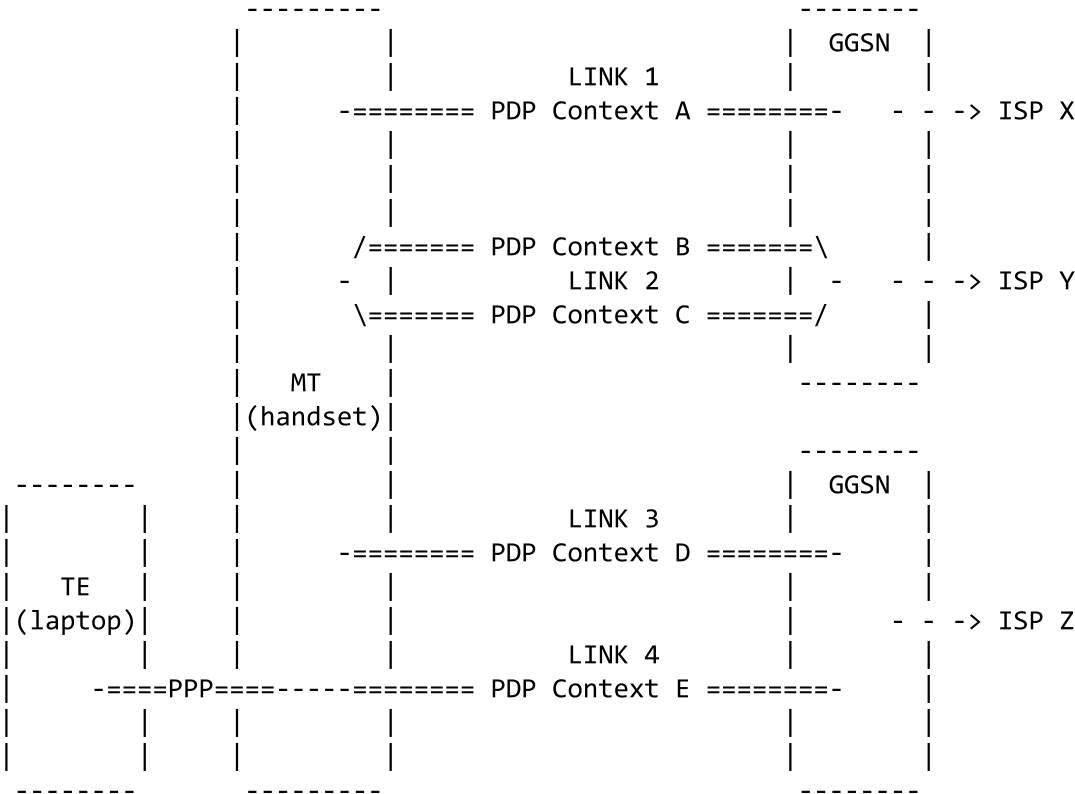
Figure 3: Correspondence of PDP Contexts to IPv6 Links
