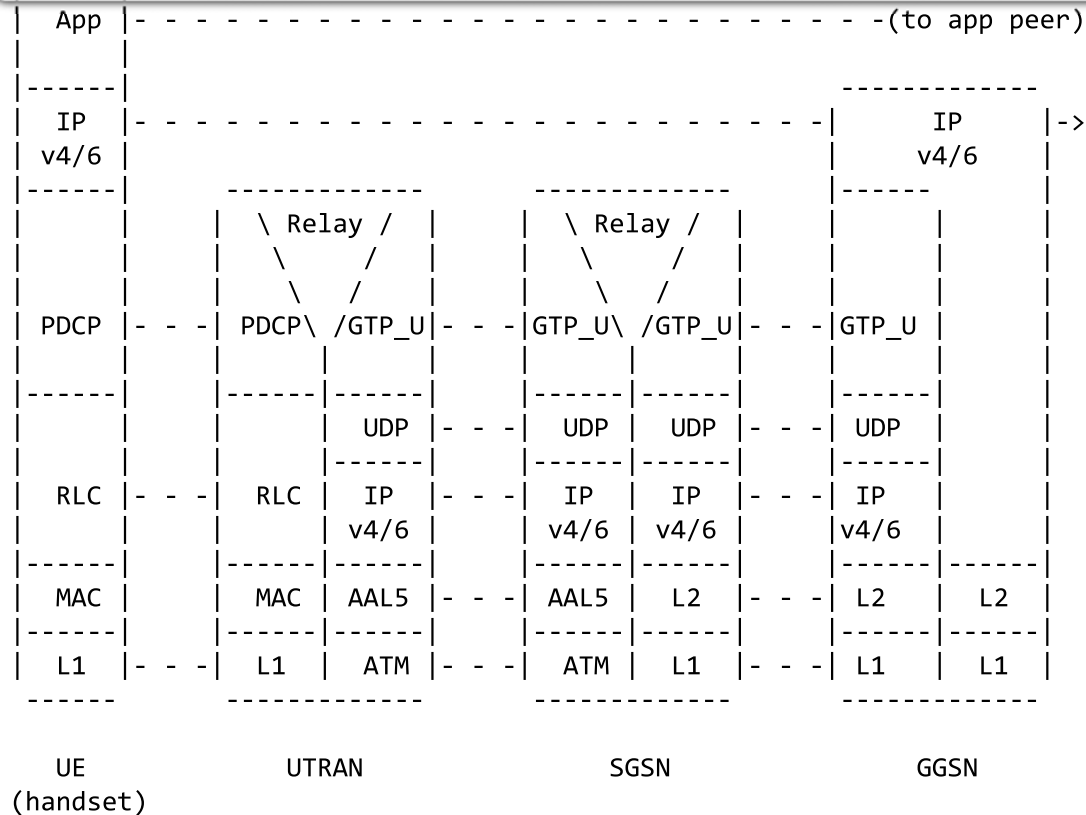
Figure 2: GPRS Protocol Stacks
