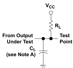
Figure 3. Load Circuit, For Open-Collector Outputs
