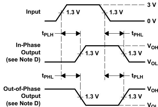
Figure 7. Voltage Waveforms, Propagation Delay Times
