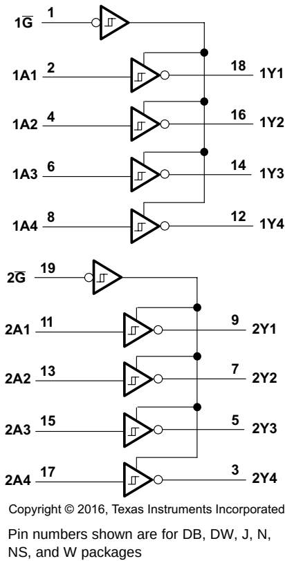
Figure 16. SNx4LS240 and SNx4S240 Logic Diagram
