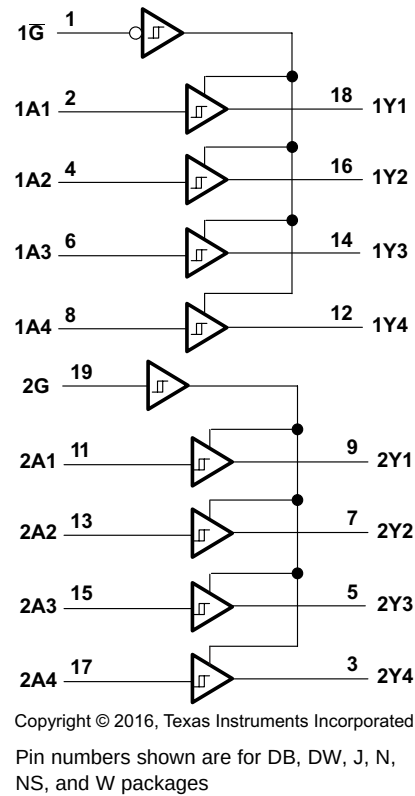
Figure 17. SNx4LS241 and SNx4S241 Logic Diagram
