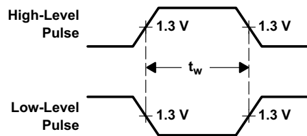
Figure 5. Voltage Waveforms, Pulse Durations
