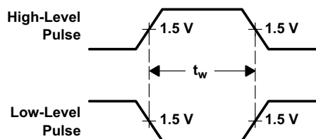
Figure 12. Voltage Waveforms, Pulse Durations
