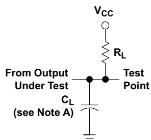
Figure 10. Load Circuit, For Open-Collector Outputs
