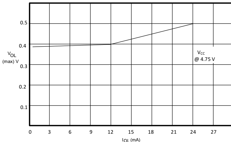
Figure 23. V_{OL} vs I_{OL}
