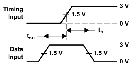
Figure 13. Voltage Waveforms, Setup and Hold Times
