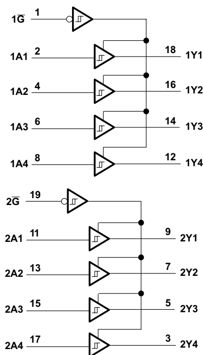
Figure 18. SNx4LS244 and SNx4S244 Logic Diagram
