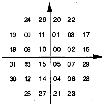
Figure 16 – Constellation labels for b = 5
