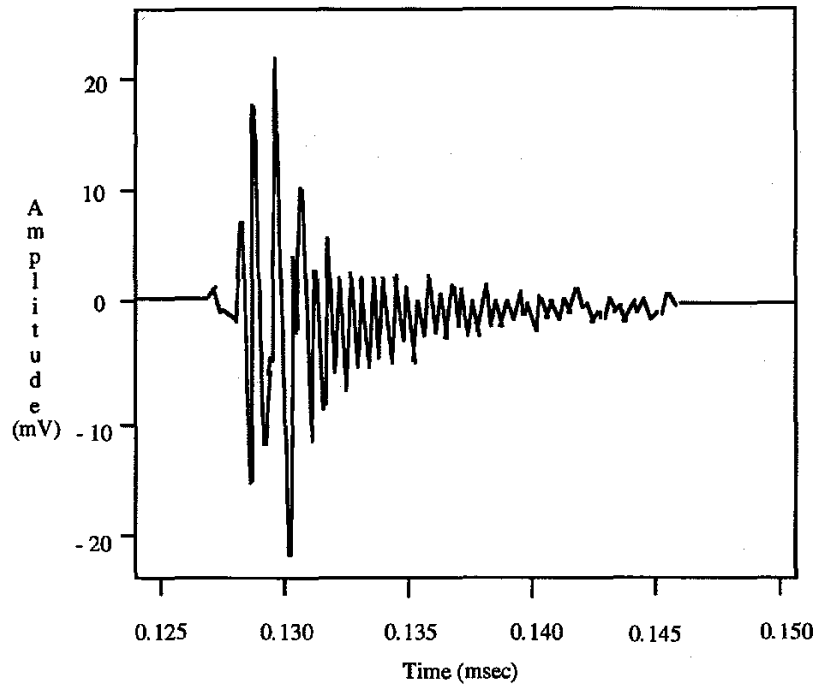
Figure 39 – Test impulse #1
