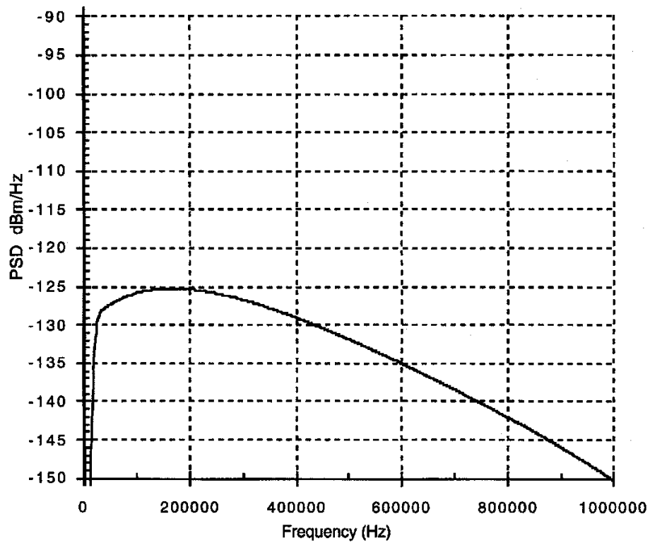
Figure B.4 – Theoretical 10-disturber ADSL FEXT
