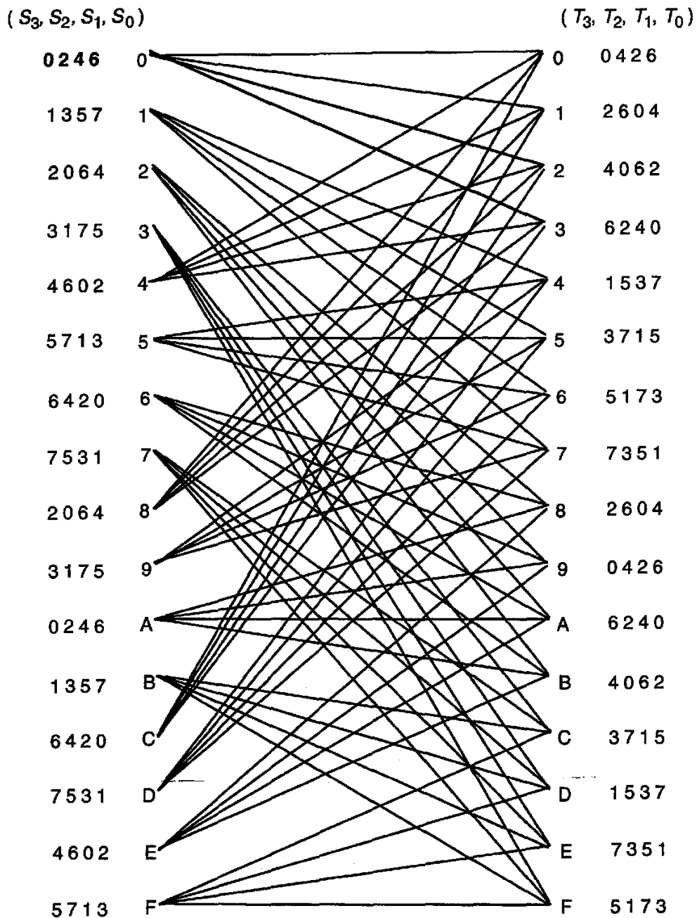
Figure 12 - Trellis diagram
