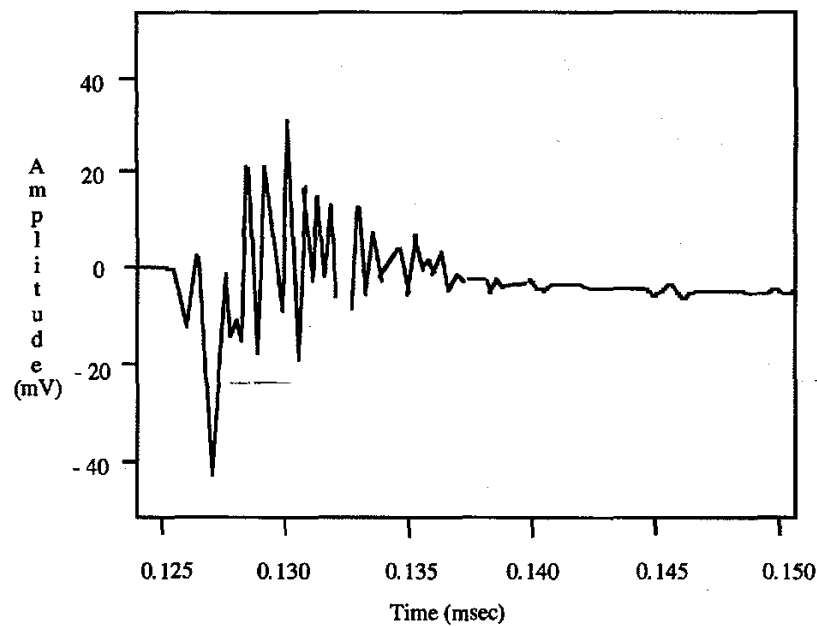
Figure 40 – Test impulse #2
