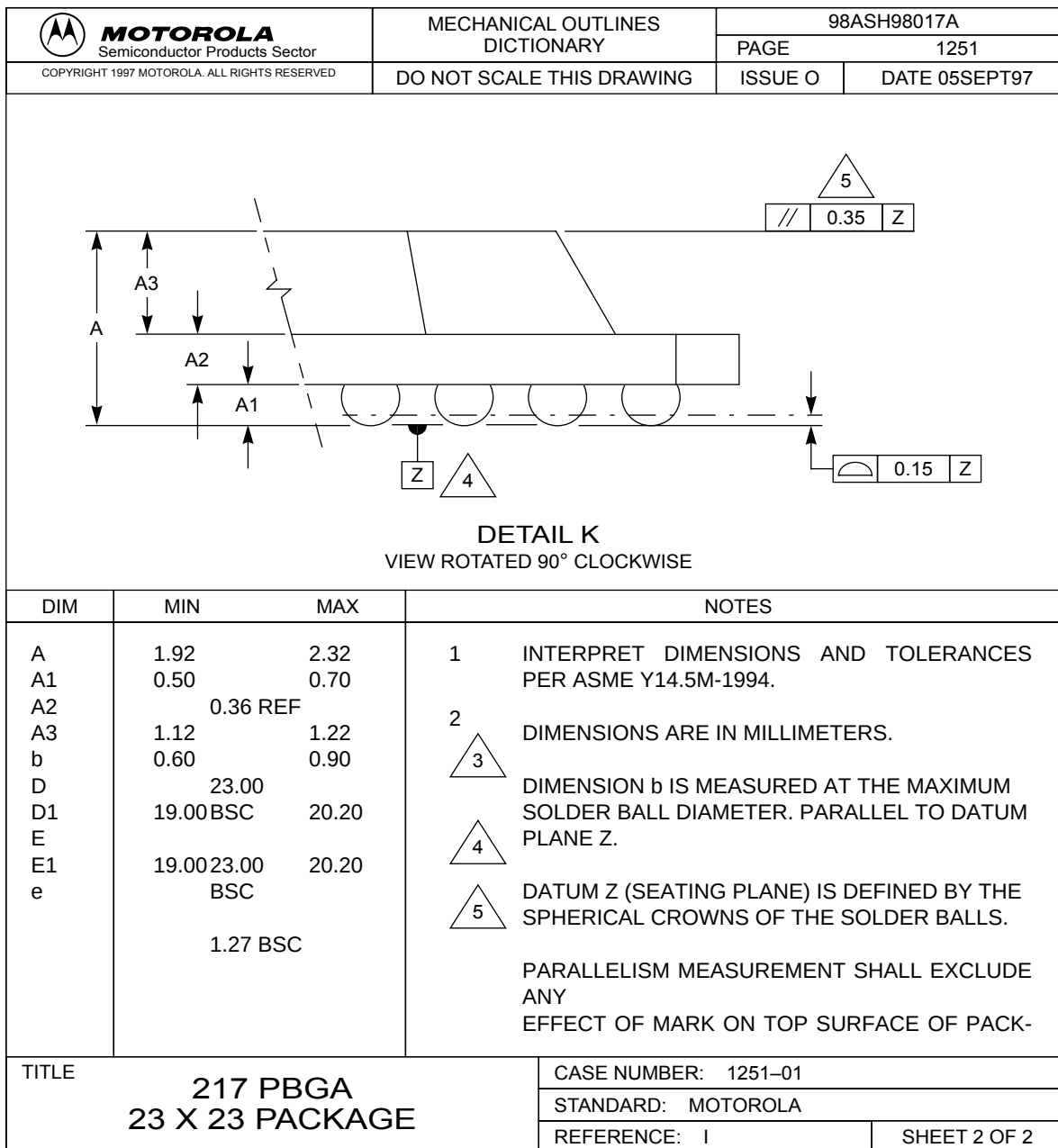
Figure 7-5. 217 PBGA Dimensions
