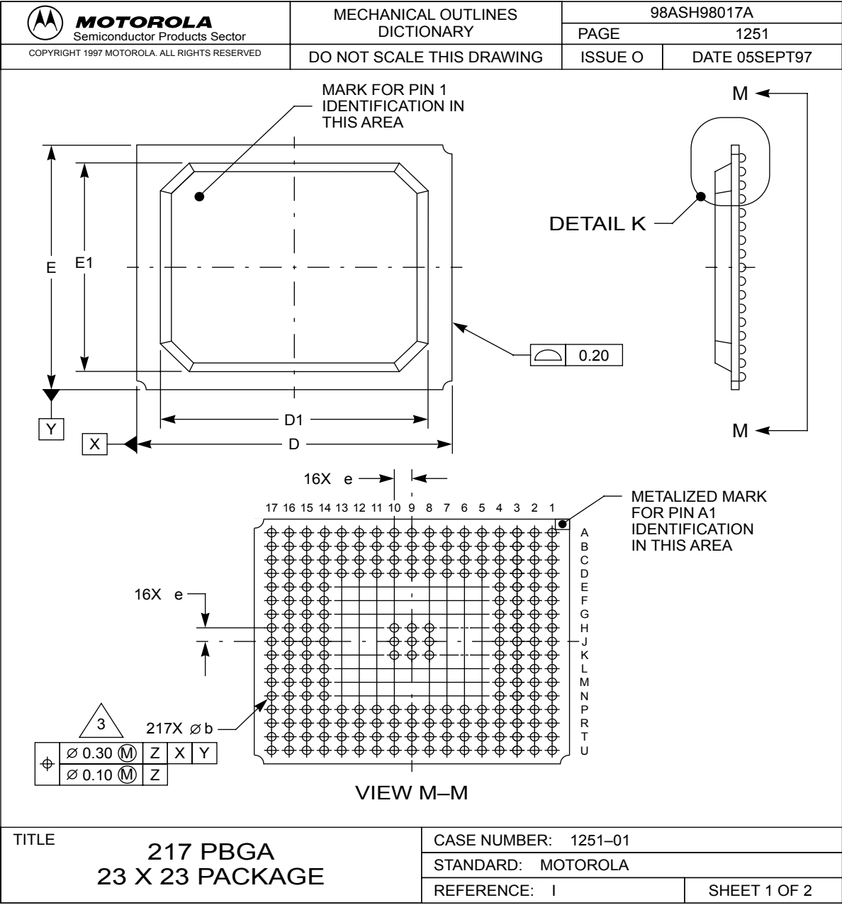
Figure 7-4. 217 PBGA Nomenclature
