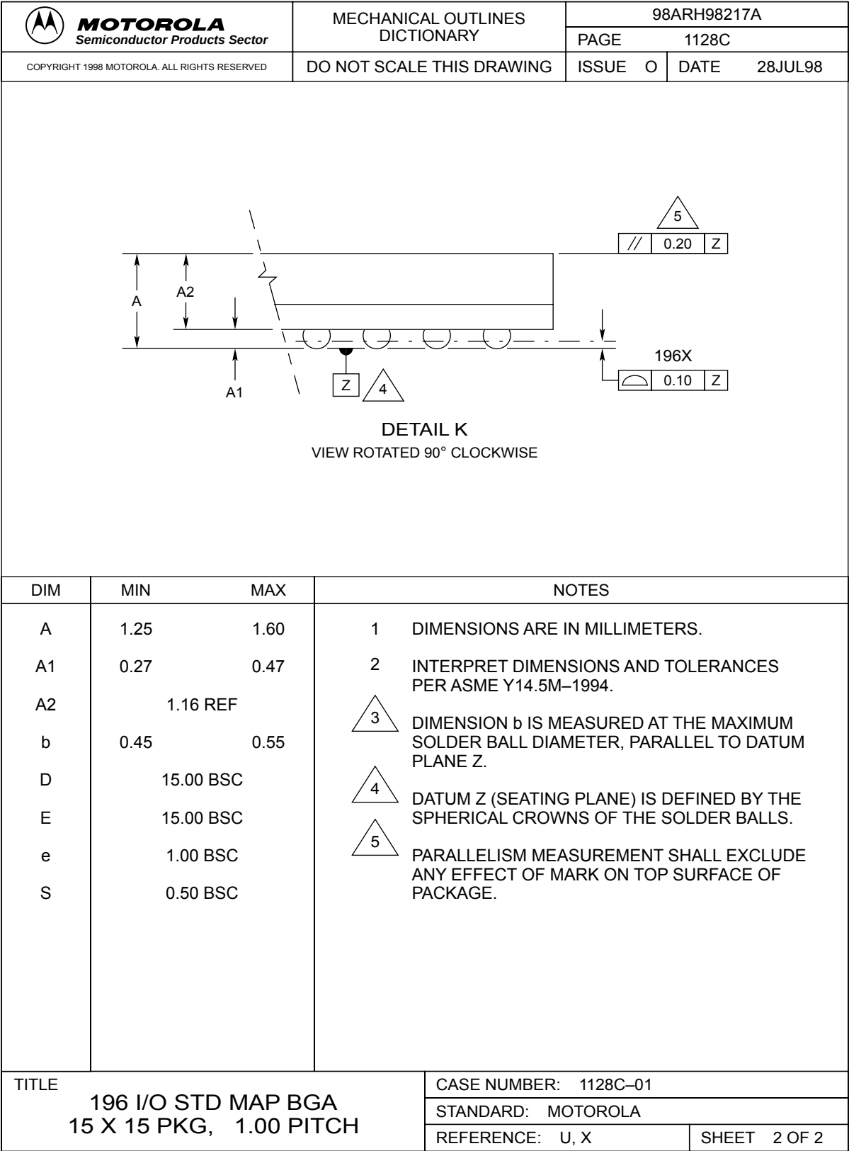
Figure 7-2. 196 MAPBGA Dimensions
