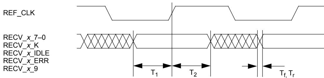
Figure 6-3. Receiver Interface Timing Diagram (DDRE = Low, RCCE = Low)
