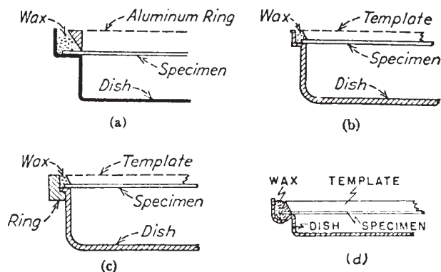
FIG. X1.2 Several Types of Dishes for Water Vapor Transmission Tests of Materials in Sheet Form
