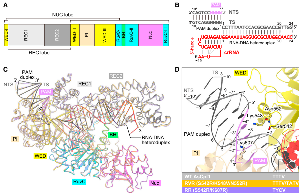
Figure 2. Overall Structure of the AsCpf1 Variant
