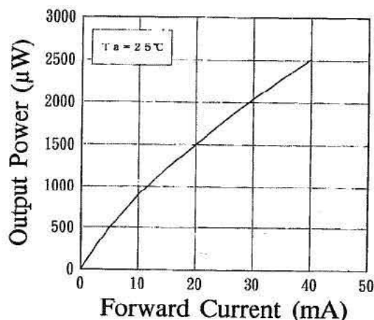
FIG. 3. The output power of the InGaN/AlGaN double-heterostructure blue LED as a function of the forward current.
