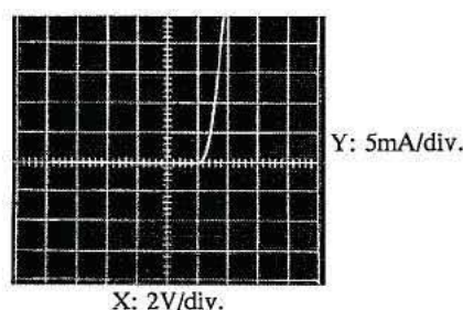
FIG. 4. Typical I - V characteristic of the InGaN/AlGaN double-heterostructure blue LED.
