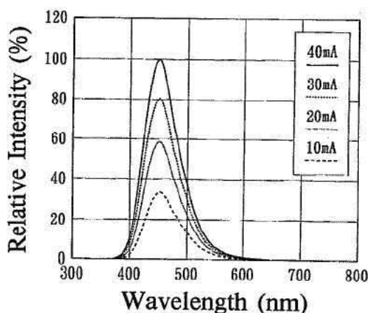
FIG. 2. Electroluminescence spectra of the InGaN/AlGaN double-heterostructure blue LED under different dc currents.
