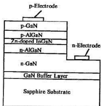
FIG. 1. The structure of the InGaN/AlGaN double-heterostructure blue LED.
