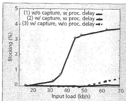
Figure 18. Capture and processing delay effect: blocking comparison.
