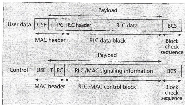
■ Figure 6. GPRS radio block structure.
