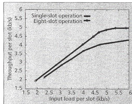
■ Figure 13. Multislot vs. single-slot operation: throughput comparison.
