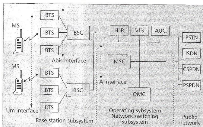
Figure 1. GSM system architecture.
