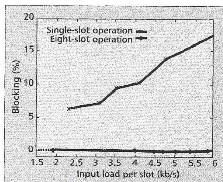
■ Figure 15. Multislot vs. single-slot operation: blocking comparison.
