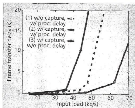
Figure 17. Capture and processing delay effect: delay comparison.
