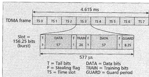
■ Figure 2. GSM burst structure.
