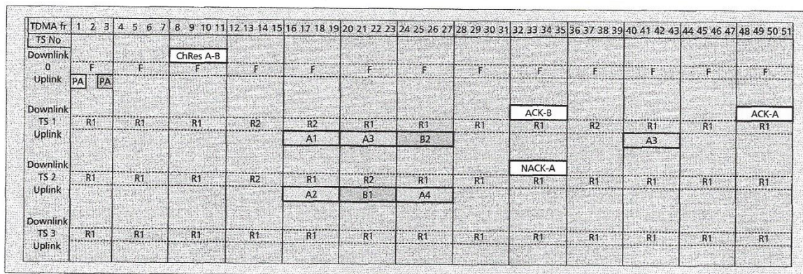
■ Figure 10. Message sequence across the air interface for mobile-originated traffic.
