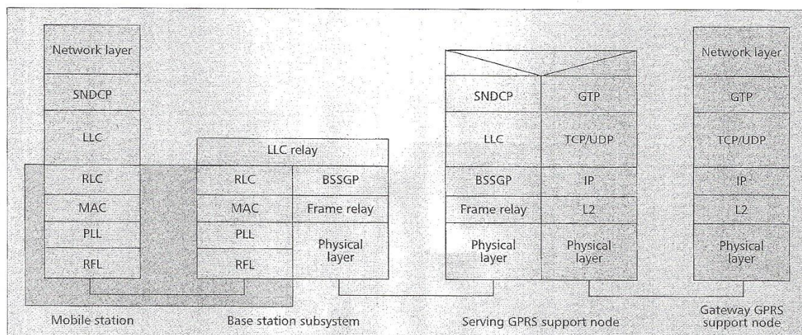
■ Figure 5. GPRS transmission plane.
