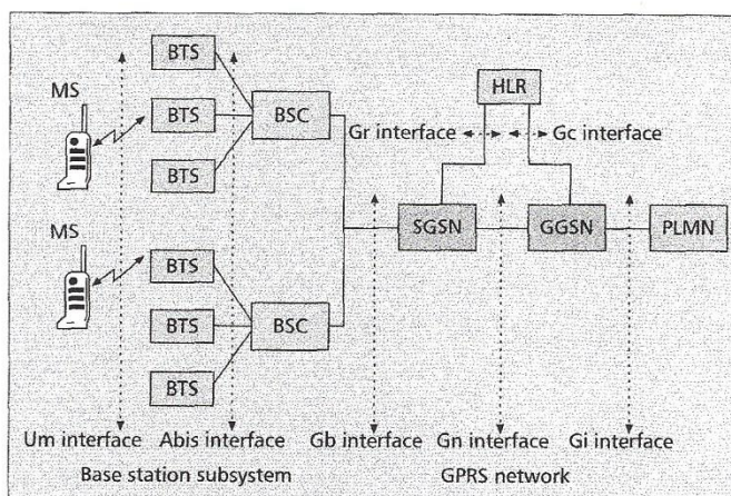
■ Figure 3. GPRS system architecture.
