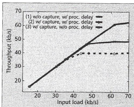
■ Figure 16. Capture and processing delay effect: throughput comparison.
