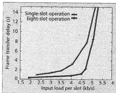
■ Figure 14. Multislot vs. single-slot operation: delay comparison.
