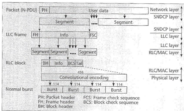
■ Figure 8. Packet transformation data flow.
