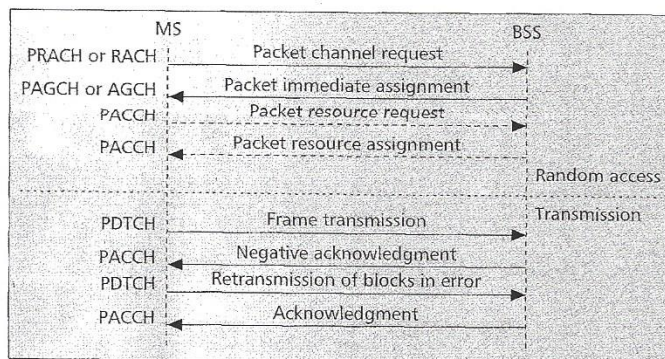
■ Figure 9. MAC layer: random access and transmission for uplink data transfer.
