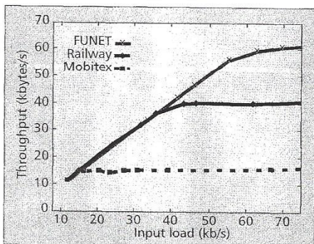
Figure 19. Traffic model effects: throughput comparison.
