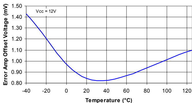
Error Amp Offset Voltage vs Temperature
