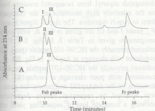
Fig. 5. Hydrophobic interaction chromatography after papain digestion of material collected by cation exchange. Approximately 20 \mu g were injected. (A) IEX-3. (B) IEX-1. (C) IEX-4.
