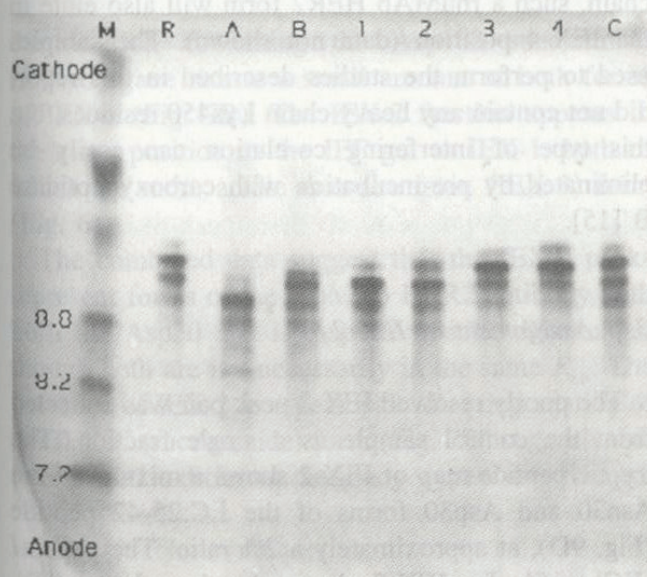
Fig. 6. Isoelectric focusing in a polyacrylamide gel. Approximately 5 \mu g of each cation-exchange fraction were loaded. Approximate pI values for the standards are given at the left. (M) IEF standards. (R) unfractionated rhuMab HER2. (A) IEX-A. (B) IEX-B. (1) IEX-1. (2) IEX-2. (3) IEX-3. (4) IEX-4. (C) IEX-C.
