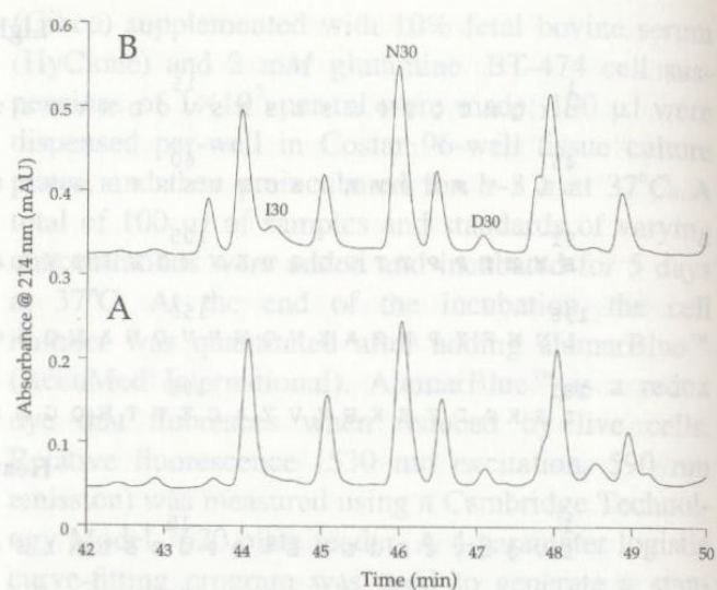
Fig. 4. Tryptic peptide map detail for stability samples. (A) control (2–8°C) sample. (B) sample stored at 30°C for 90 days in a pH 5 acetate-NaCl excipient.
