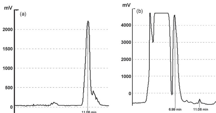
Fig. 3. Preparative chromatograms obtained with Waters SymmetryPrep \text{C}_{18} (7.8 mm \times 300 mm; 7 \mu\text{m} ). (a) Detection with a NaI(Tl) detector. (b) Detection with a UV detector at 265 nm.
