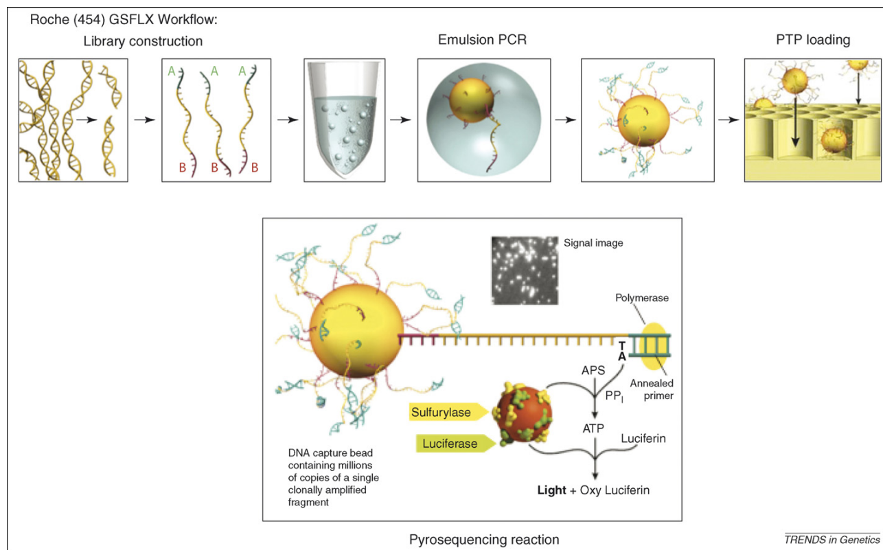
Figure 1. 454 Workflow: library construction ligates 454-specific adapters to DNA fragments and couples amplification beads with DNA in an emulsion PCR to amplify fragments before sequencing. The beads are loaded into the picotiter plate (PTP). The bottom panel illustrates the pyrosequencing reaction that occurs on nucleotide incorporation to report sequencing by synthesis.
