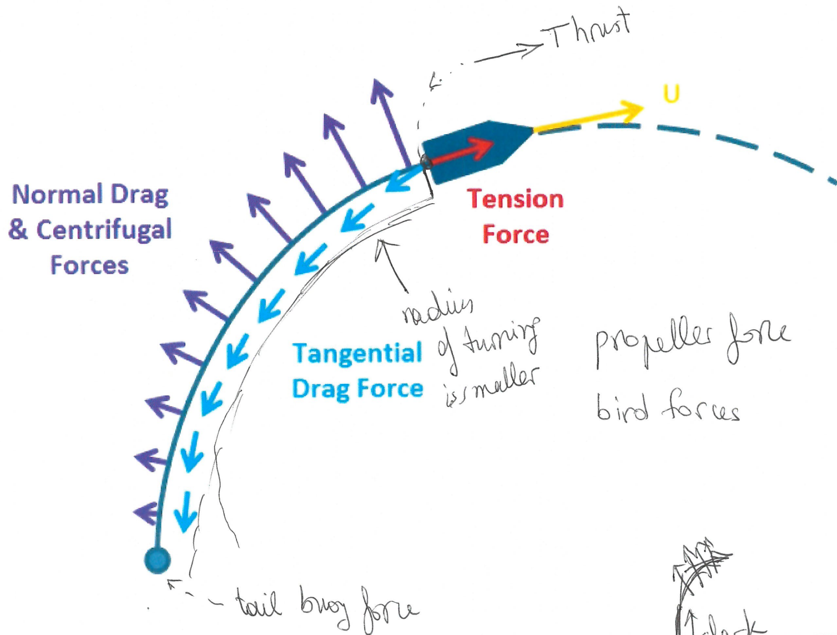
Figure 6 - The forces on a seismic streamer during a turn.
