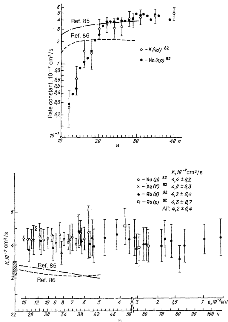
FIG. 15. Rate constant for charge transfer from a Rydberg atom to a molecule of \text{SF}_6 as measured for different values of the principal quantum number n of Rydberg atoms of different types. 82,83 Also presented are the results of calculating the rate constant of the process 85 \text{Rb}(n) + \text{SF}_6 \rightarrow \text{Rb}^+ + \text{SF}_6^- (dotted line) and the rate constant for capture of a slow electron at an electron energy equal to the mean kinetic energy of an electron in a Rydberg atom with the given value of n 86 (dotted line). a—Small n . b—Large n .
