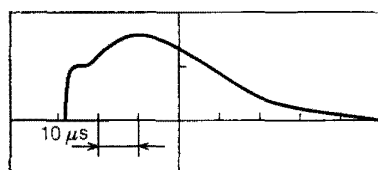
FIG. 9. Oscillogram of the photocurrent observed in two-photon laser excitation of Na vapor ( \lambda = 578.9 \text{ nm} ). 35
