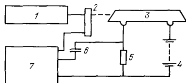
FIG. 17. Typical diagram of an optogalvanic experiment. 1—tunable laser; 2—modulator; 3—gas-discharge tube; 4—power supply; 5—ballast resistor; 7—amplifier.
