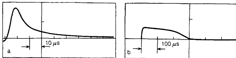
FIG. 8. Oscillogram of the photocurrent that arises upon irradiating a discharge tube containing a mixture of Na + Ne with a pulse of laser radiation ( \lambda = 589 \text{ nm} ), 35 in the presence of a discharge (a), and at a voltage below that for ignition of the discharge (b).
