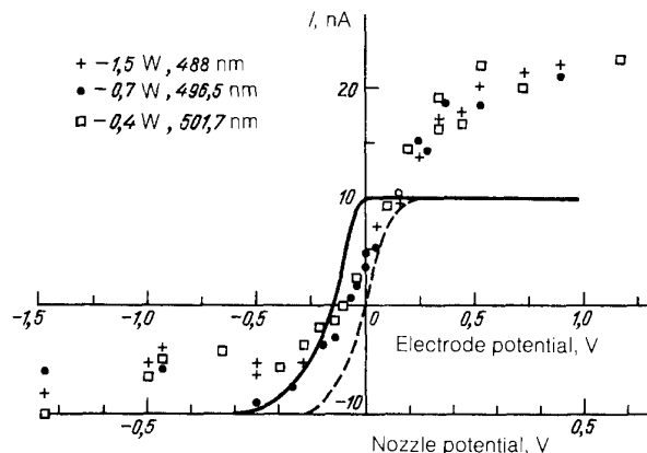
FIG. 11. Dependences of the photocurrent of Cs ^{+} ions on the extracting potential obtained using a continuous-wave laser of varying power and wavelength. 18
