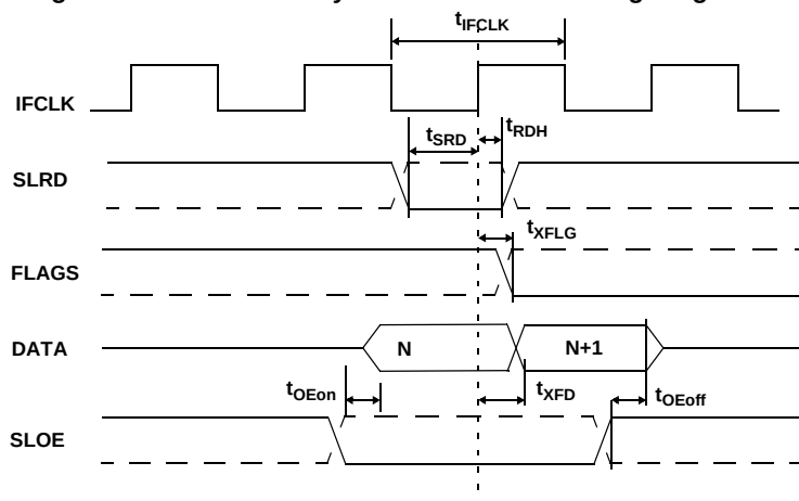
Figure 9-7. Slave FIFO Synchronous Read Timing Diagram [21]
