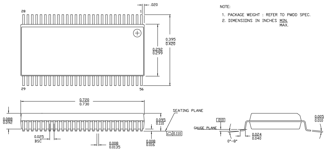
Figure 11-1. 56-Pin Shrunk Small Outline Package O56 (51-85062)
