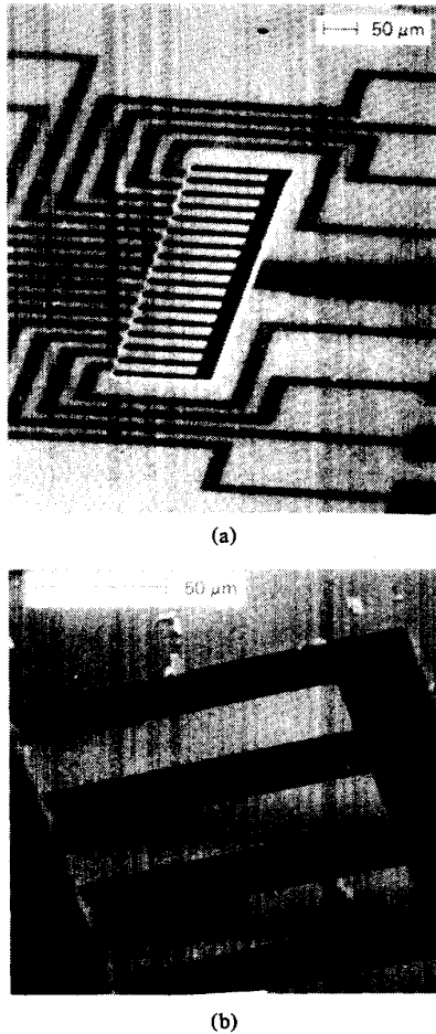
Fig. 47. SEM photographs of a completed 16-element light modulator array, ready for bonding. Note the high degree of flatness and uniformity of the beams. The \text{SiO}_2 beams are 100 \mu\text{m} long, 25 \mu\text{m} wide, and 0.5 \mu\text{m} thick.
