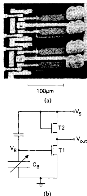
Fig. 55. The integrated accelerometer shown here in (a) consists of an SiO 2 cantilever beam sensor (loaded with a gold mass for increased sensitivity) coupled to an MOS detection circuit. The capacitance of the beam (typically 3.5 fF) is employed in a voltage divider network (b) from which small variations in the beam capacitance drive the detection transistor. From [170].
