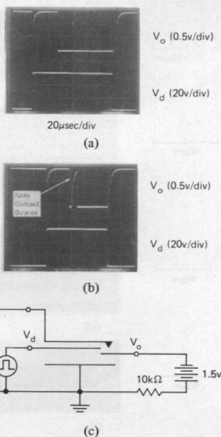
Fig. 60. (a) and (b) Oscilloscope traces of typical pulsed switching behavior for the circuit shown in (c). The deflection voltage in (a) is just above the switching threshold (~60 V), while the voltage in (b) has been increased to about 62 V. Note the delay time (~40 \mu s) between the application of the deflection voltage and the actual time the switch is closed. For higher deflection voltages (shown in the second oscilloscope trace), delay times are reduced and contact bounce effects are observed.
