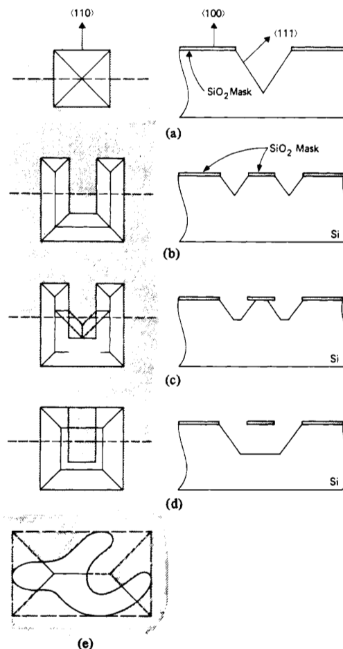
Fig. 5. (a) Typical pyramidal pit, bounded by the (111) planes, etched into (100) silicon with an anisotropic etch through a square hole in an oxide mask. (b) Type of pit which is expected from an anisotropic etch with a slow convex undercut rate. (c) The same mask pattern can result in a substantial degree of undercutting using an etchant with a fast convex undercut rate such as EDP. (d) Further etching of (c) produces a cantilever beam suspended over the pit. (e) Illustration of the general rule for anisotropic etch undercutting assuming a "sufficiently long" etching time.
